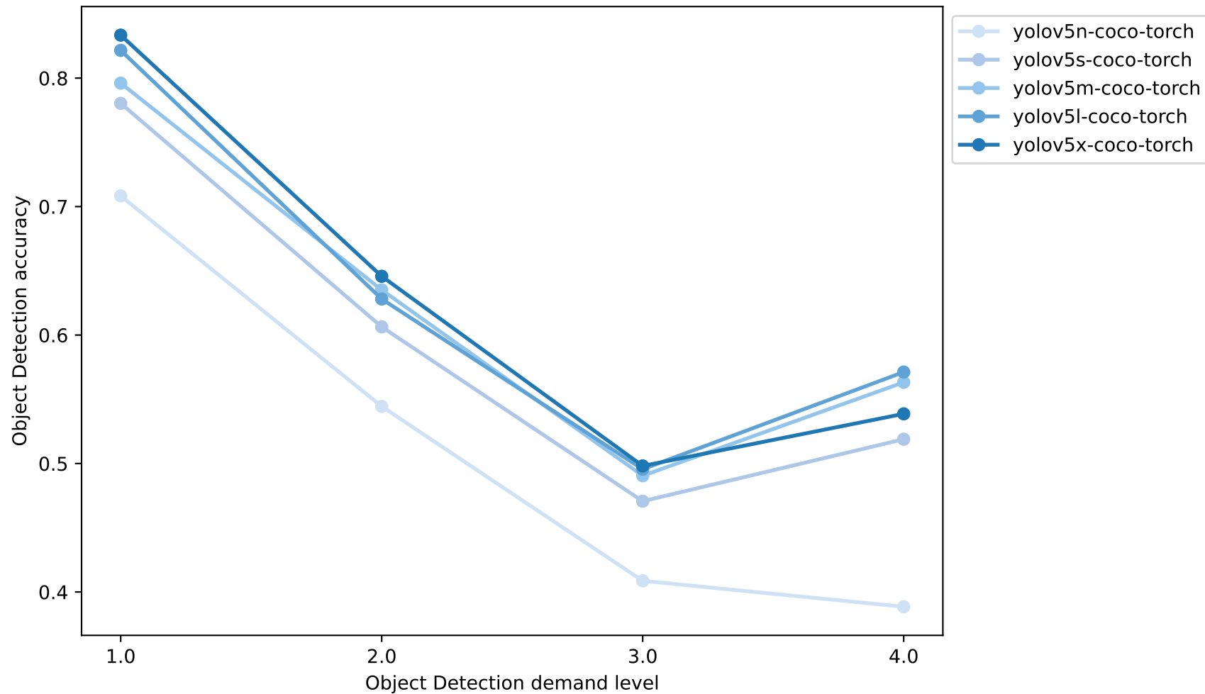
YOLOv5 Object Detection Accuracy by Demand Level — Zero-shot (calibration)
