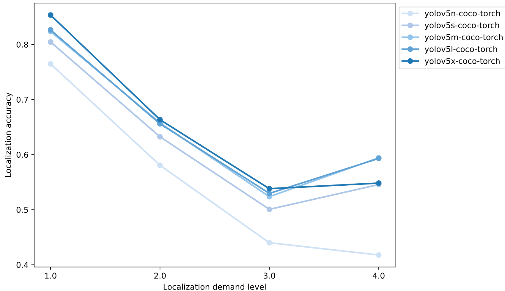
YOLOv5 Localization Accuracy by Demand Level — Zero-shot (calibration)
