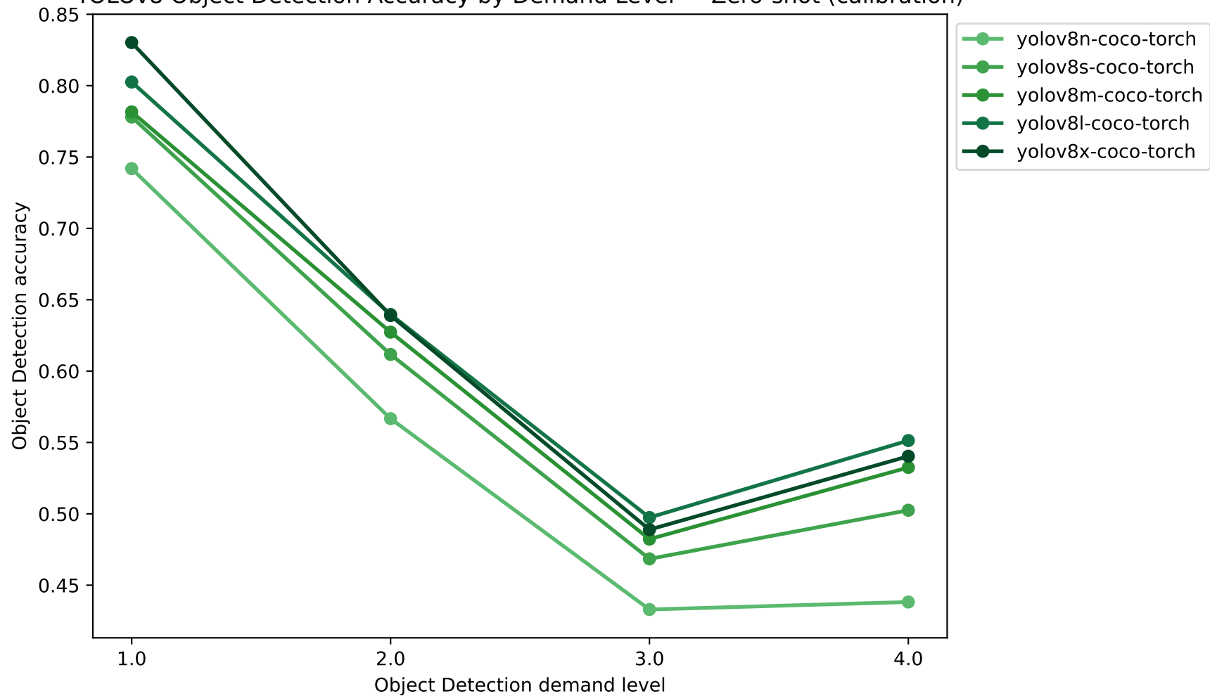
YOLOv8 Object Detection Accuracy by Demand Level — Zero-shot (calibration)
