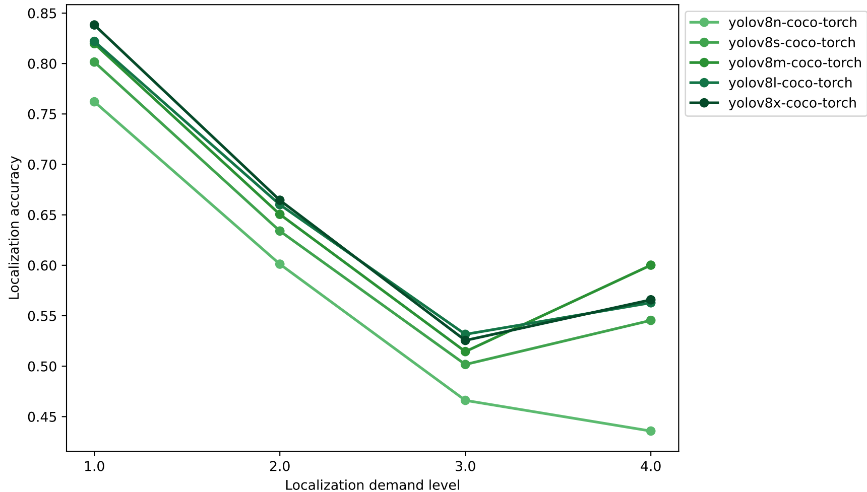
YOLOv8 Localization Accuracy by Demand Level — Zero-shot (calibration)
