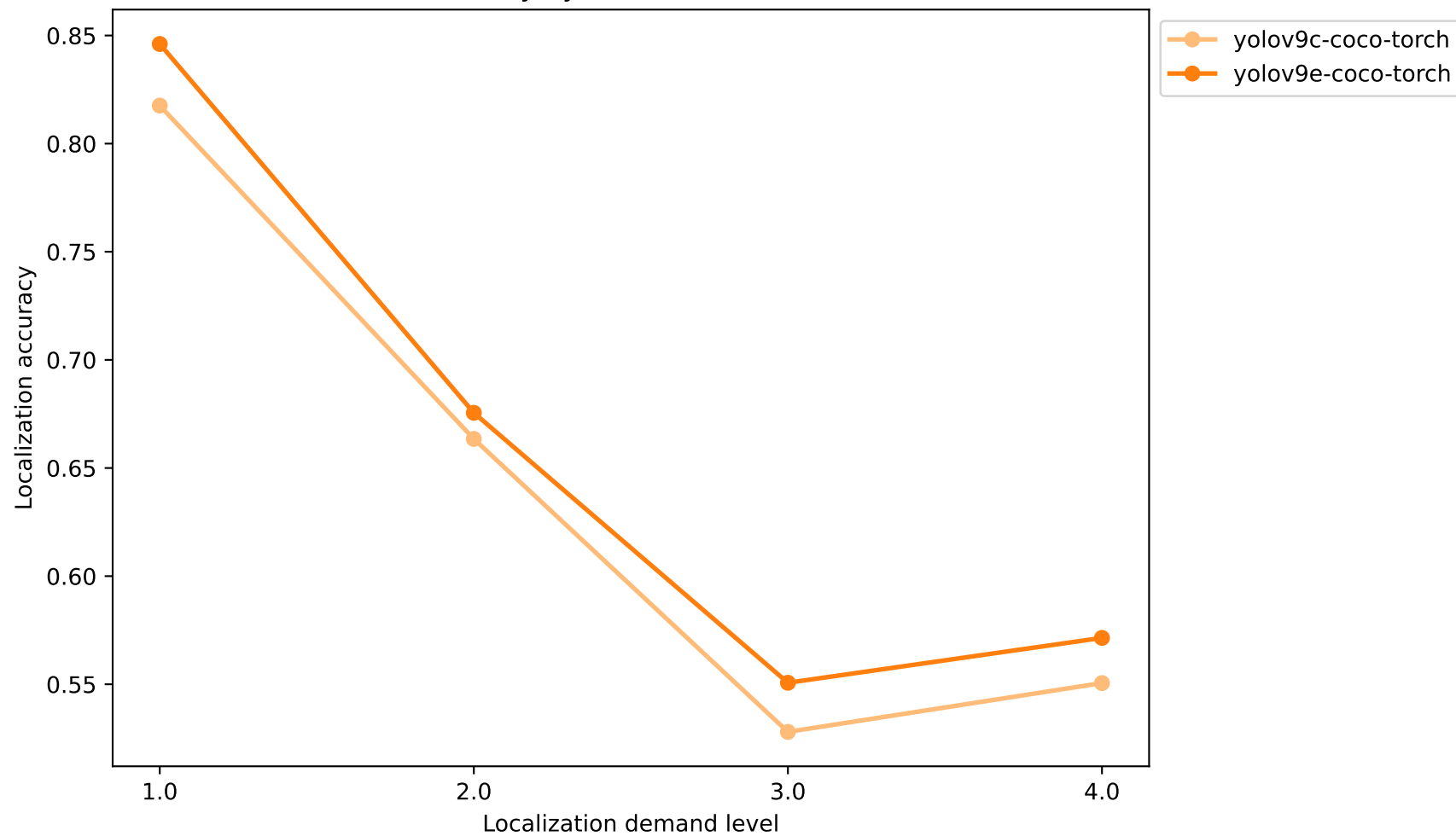
YOLOv9 Localization Accuracy by Demand Level — Zero-shot (calibration)
