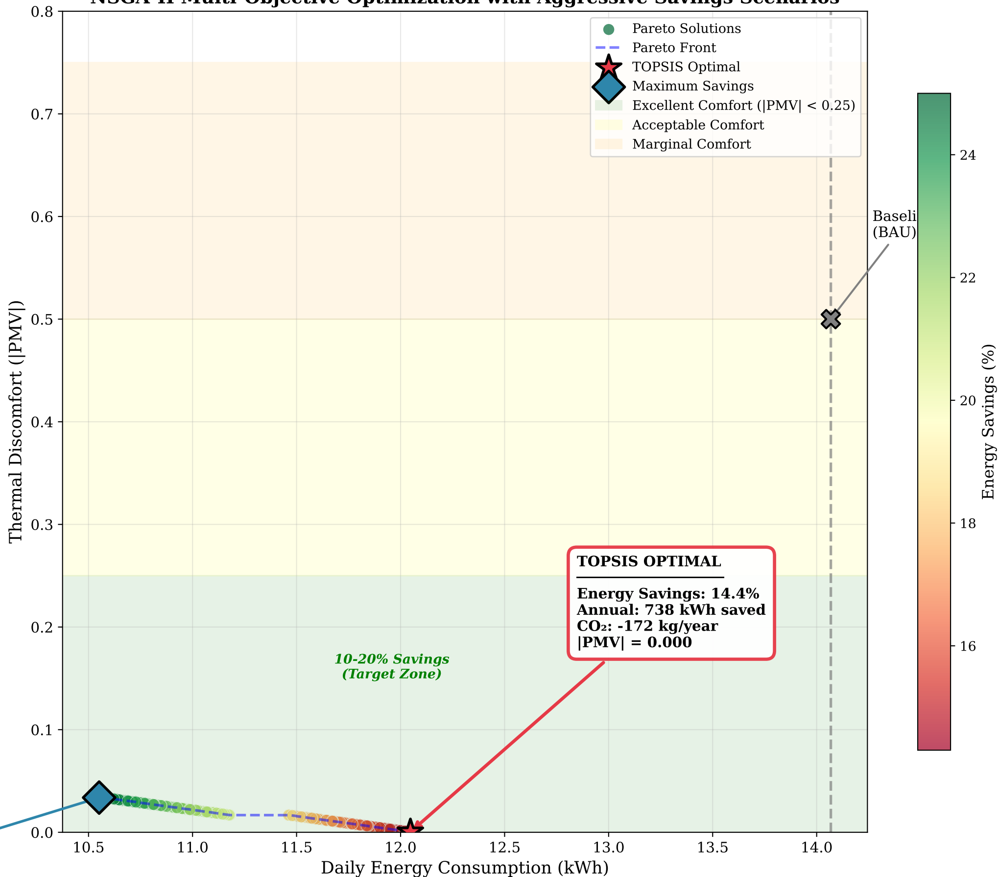
FIGURE 3: Enhanced Pareto Front - Energy vs. Comfort Trade-off NSGA-II Multi-Objective Optimization with Aggressive Savings Scenarios
