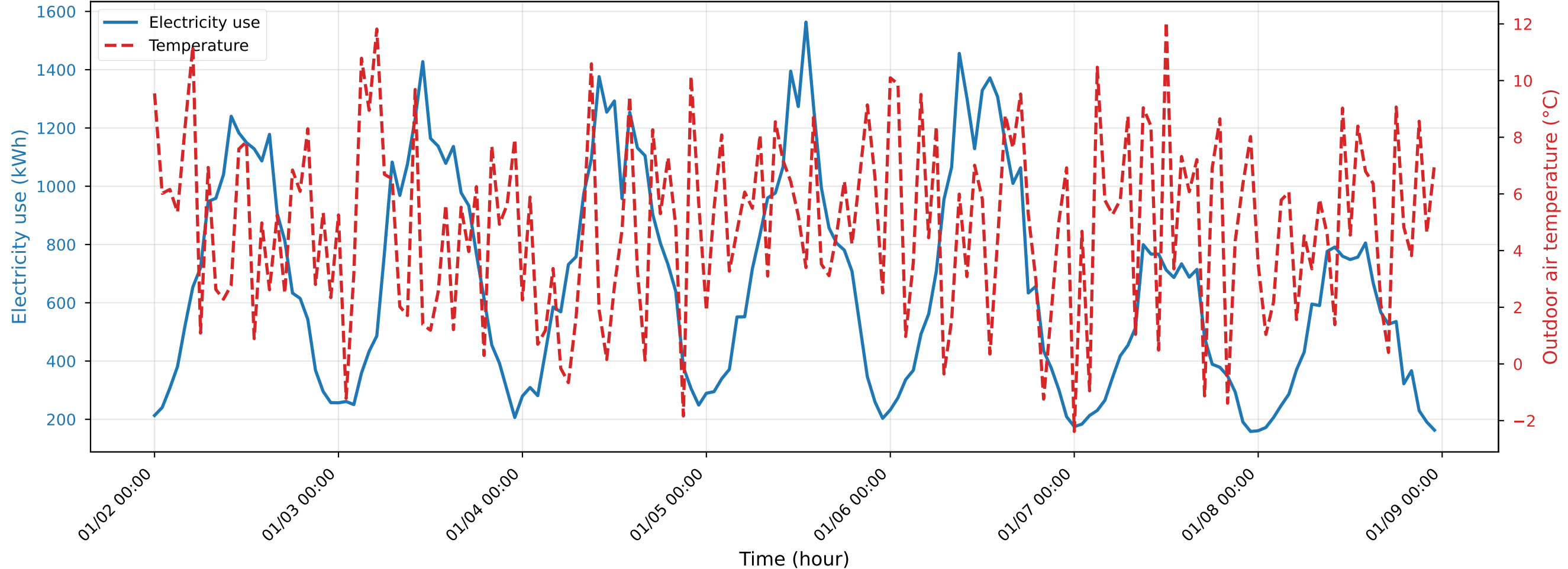
Hourly Electricity Use and Outdoor Temperature - Representative Week Office at site_2
