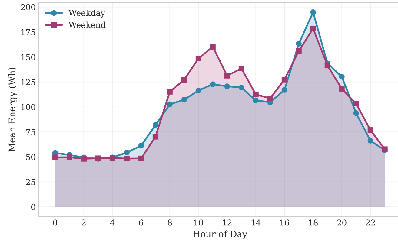
(d) Daily Consumption Pattern (Blue=Weekday, Purple=Weekend)
