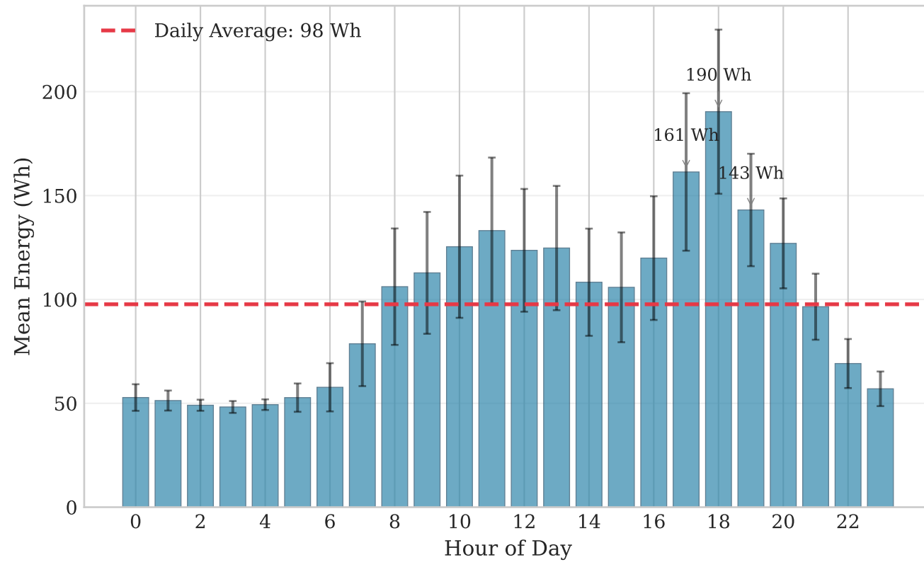
(a) Average Hourly Energy Consumption (Appliances)
