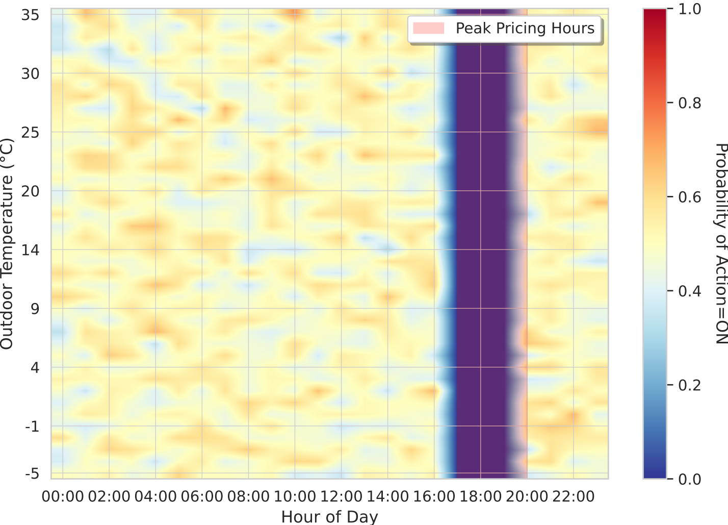
Control Policy Heatmap: Learned Demand Response Strategy
