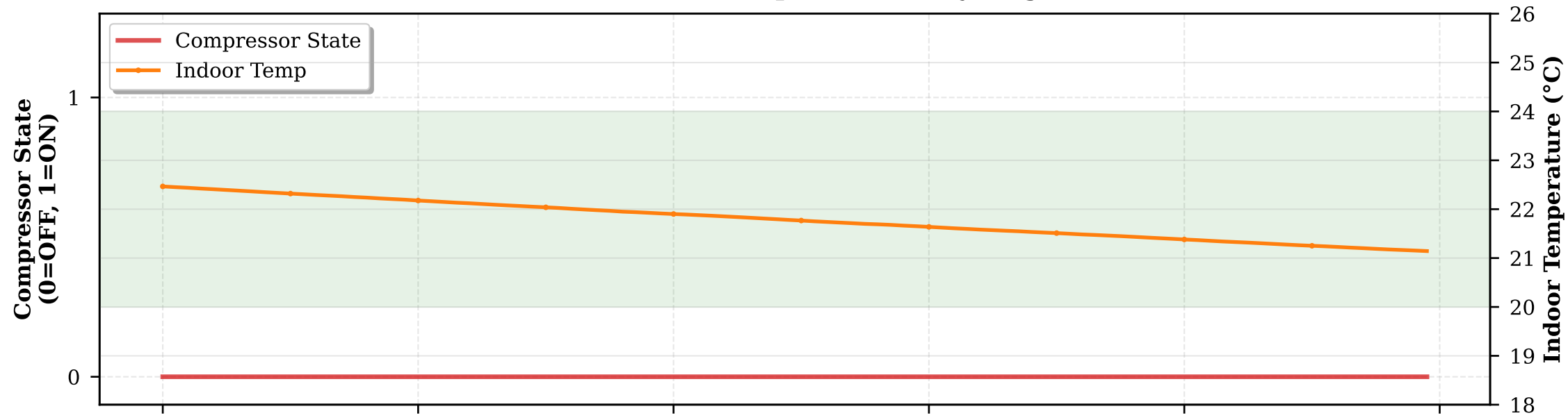
(a) Baseline Thermostat: Frequent Short-Cycling (0 switches)
