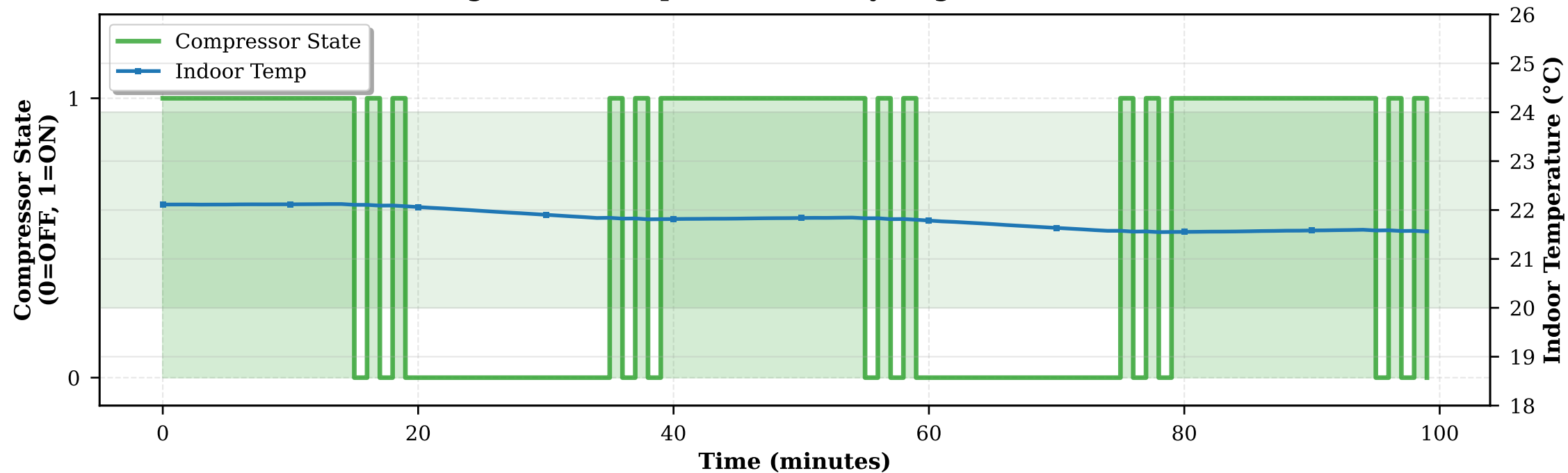
(b) PI-DRL Agent: Stable Operation with Cycling Prevention (25 switches)
