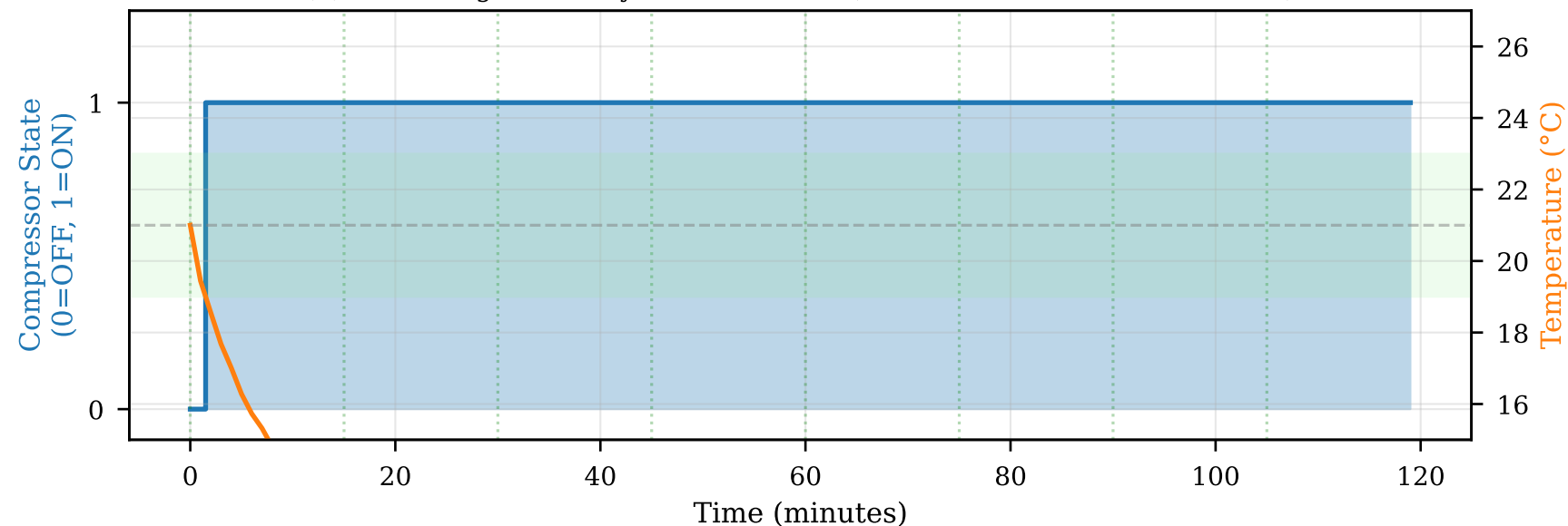
(b) PI-DRL Agent — 1 cycles in 120 min (Green lines: 15-min boundaries)
