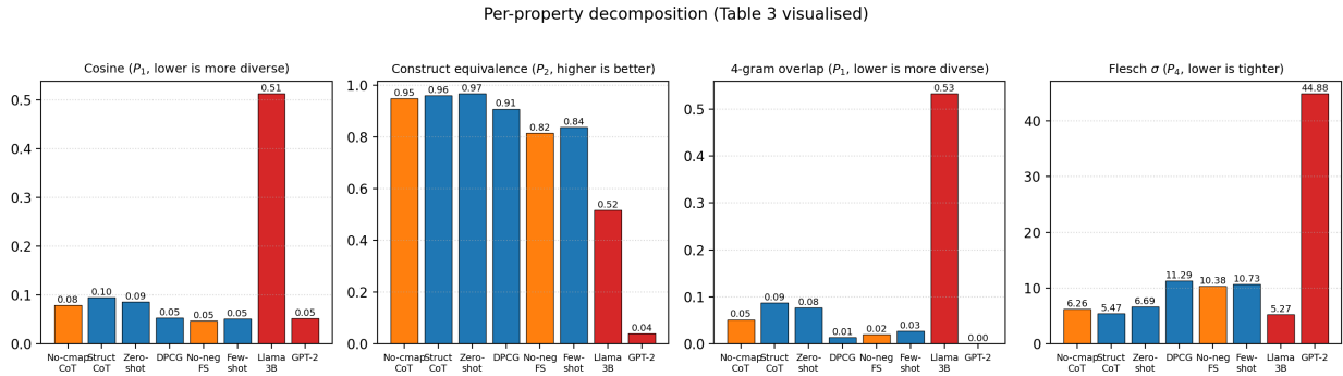
Figure 2: Per-method scores on the four AIAA properties. No single strategy dominates all four dimensions; no-negative-anchors few-shot and DPCG tie on surface diversity, structured CoT and zero-shot win on construct equivalence and readability parity.
