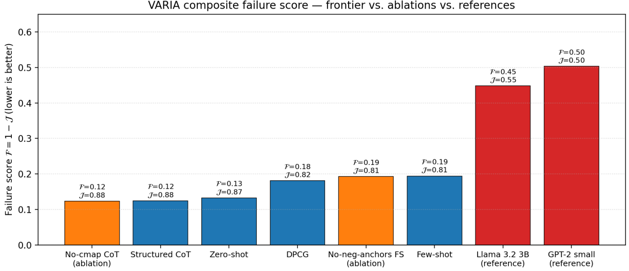
Figure 1: Composite VARIA failure score across the eight evaluated conditions. Lower is better. Frontier prompting strategies cluster between \mathcal{F} \approx 0.12 and 0.19; the Llama 3.2 3B Instruct and GPT-2 small references occupy a clearly separated regime above \mathcal{F} = 0.44 .
