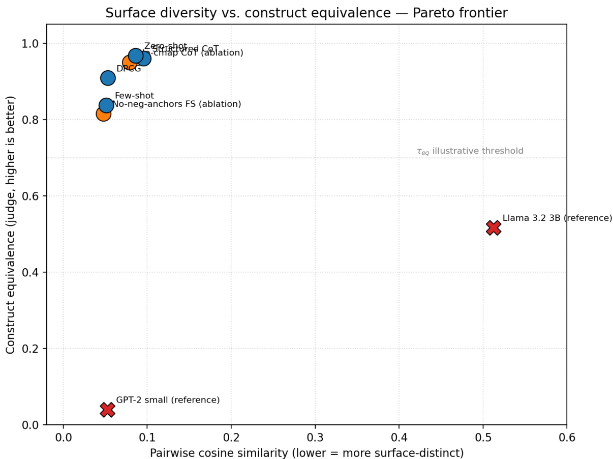
Figure 3: Surface diversity versus construct equivalence trade-off. Frontier strategies and ablations trace a Pareto frontier; the Llama 3.2 3B Instruct reference occupies a degenerate high-cosine, low-equivalence corner, while GPT-2 small sits at near-zero equivalence regardless of cosine.
