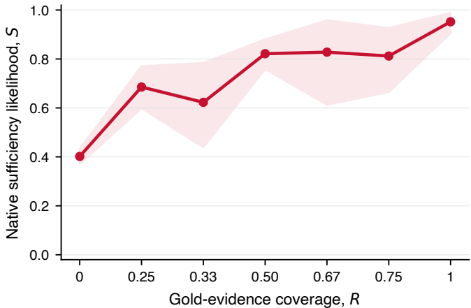
Sufficiency as a function of evidence coverage
