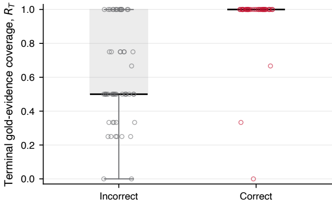
Terminal coverage by answer correctness
