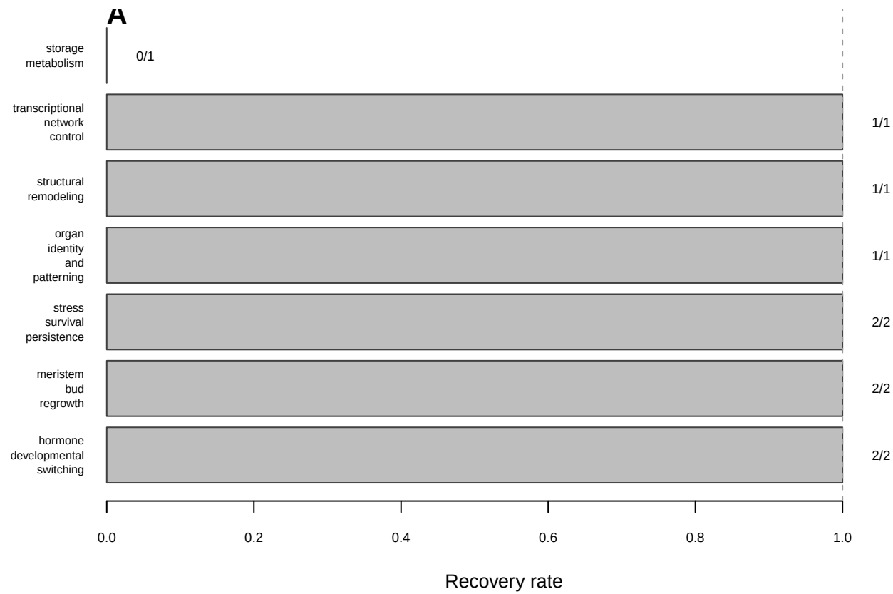
Known-category recovery
