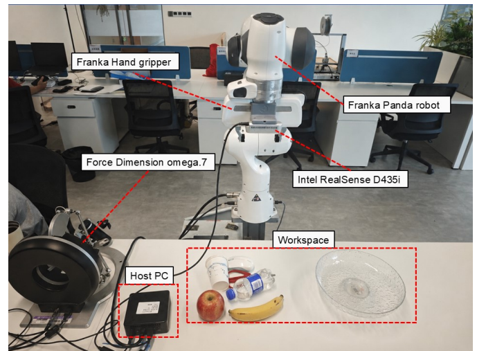
Figure 1: Experimental teleoperation platform showing the Omega.7 master device, a Franka Panda manipulator equipped with a Franka Hand gripper, the Intel RealSense D435i camera, the control computer, and the object workspace.
