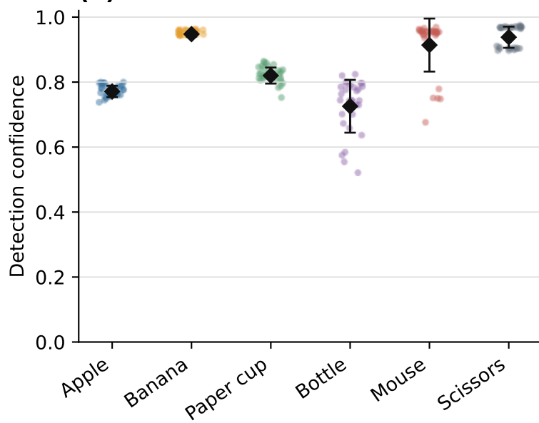
(b) Confidence
