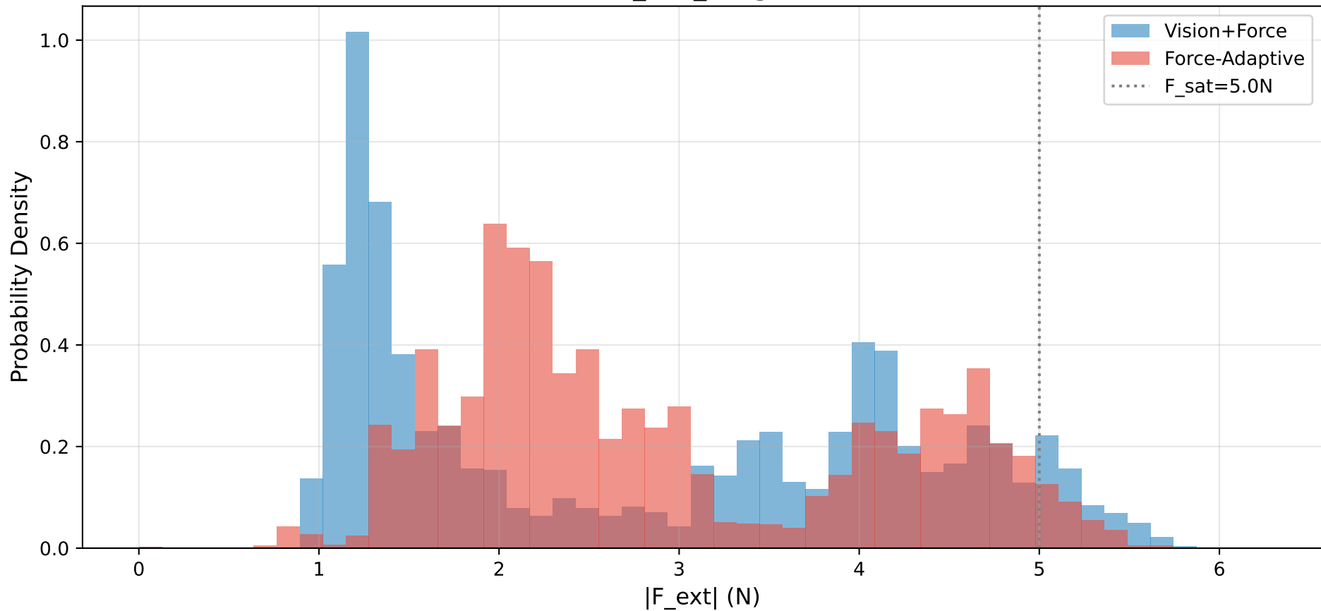
Figure 4: F_{\text{ext\_mag}}
