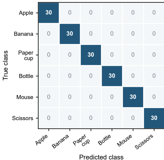
(a) Confusion matrix ( n = 180 )
