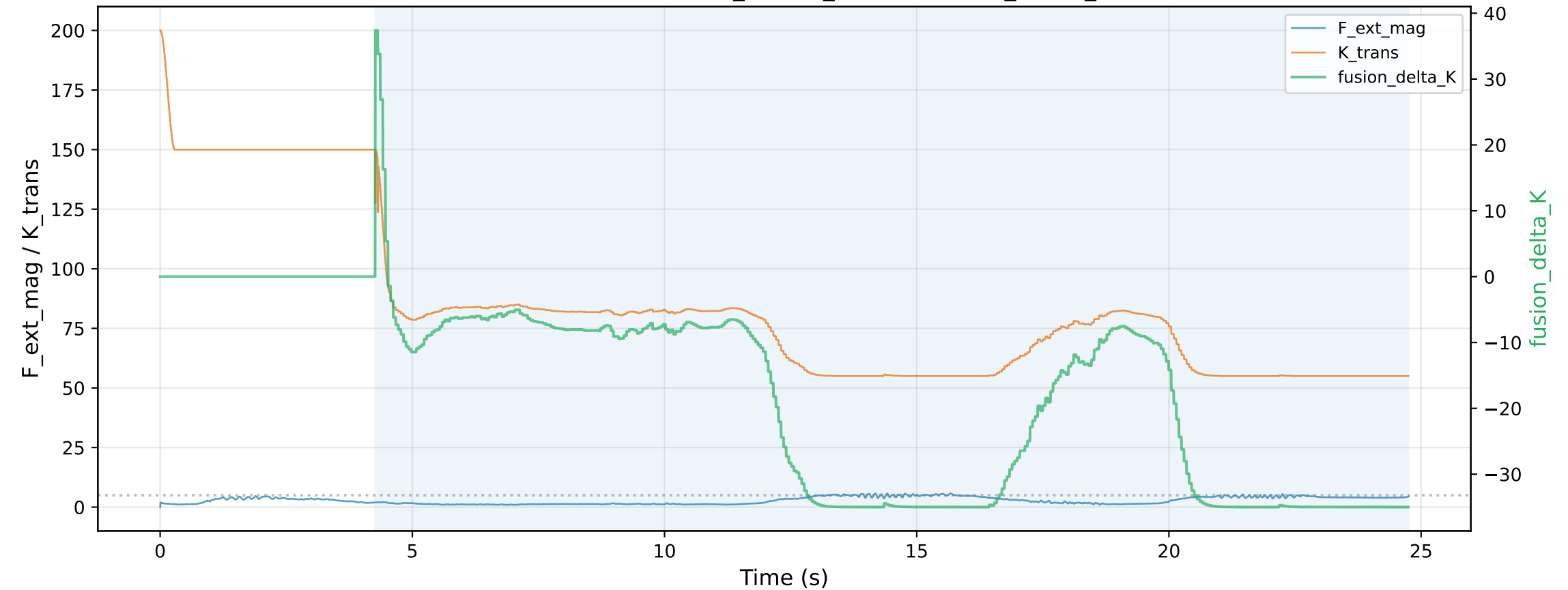
3: Vision+Force — F_ext, K_trans, fusion_delta_K
