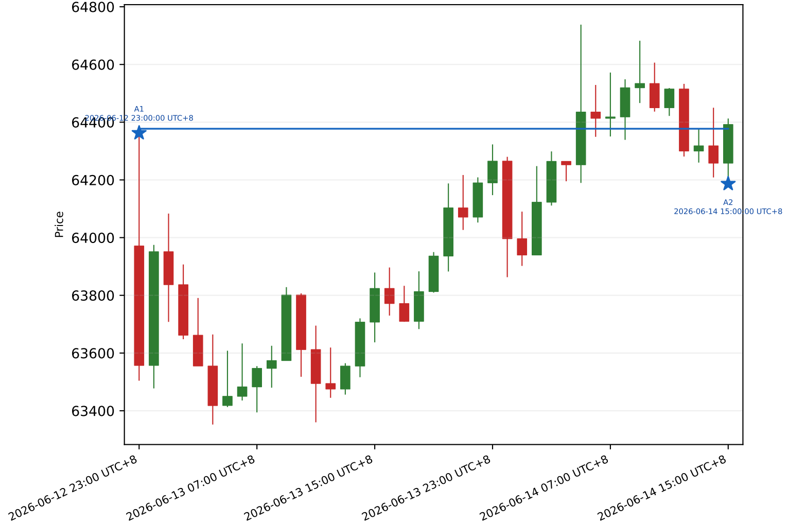
BTC 1h | PATTERN_004 Horizontal Support rule=breakout_retest | score=89.21
