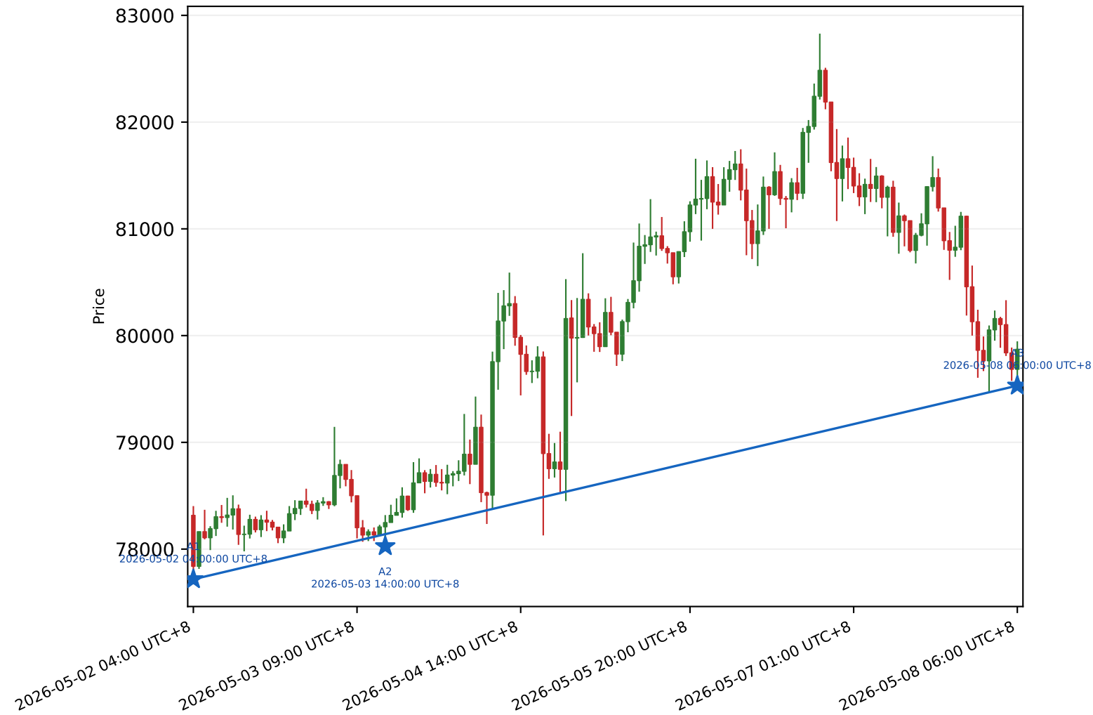
BTC 1h | PATTERN_003 Three Point Trendline Support rule=strict_three_point_slope_support | score=97.91
