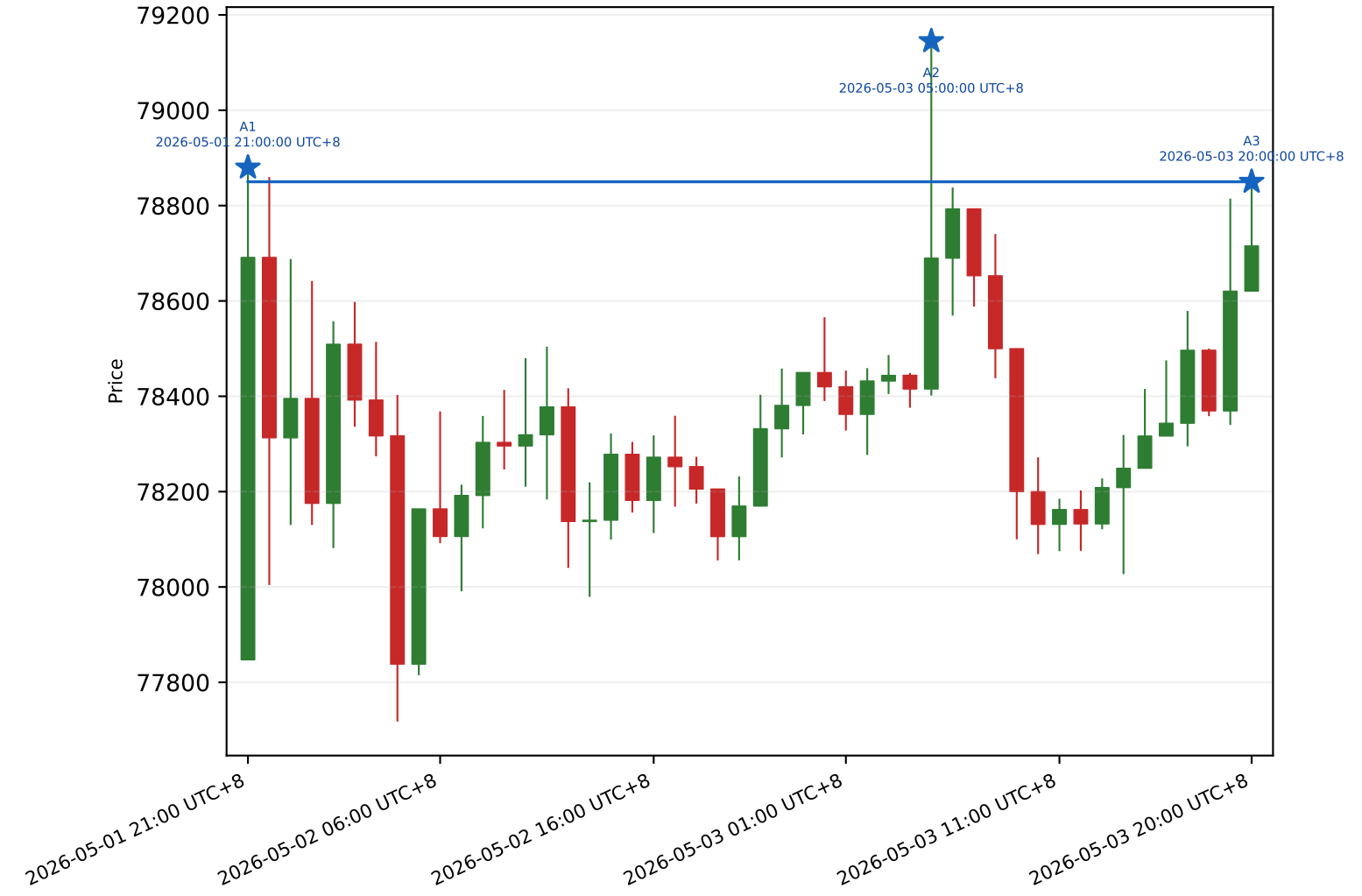
BTC 1h | PATTERN_008 Head and Shoulders Top rule=confirmed_three_swing_high_head_shoulders_top | score=73.13
