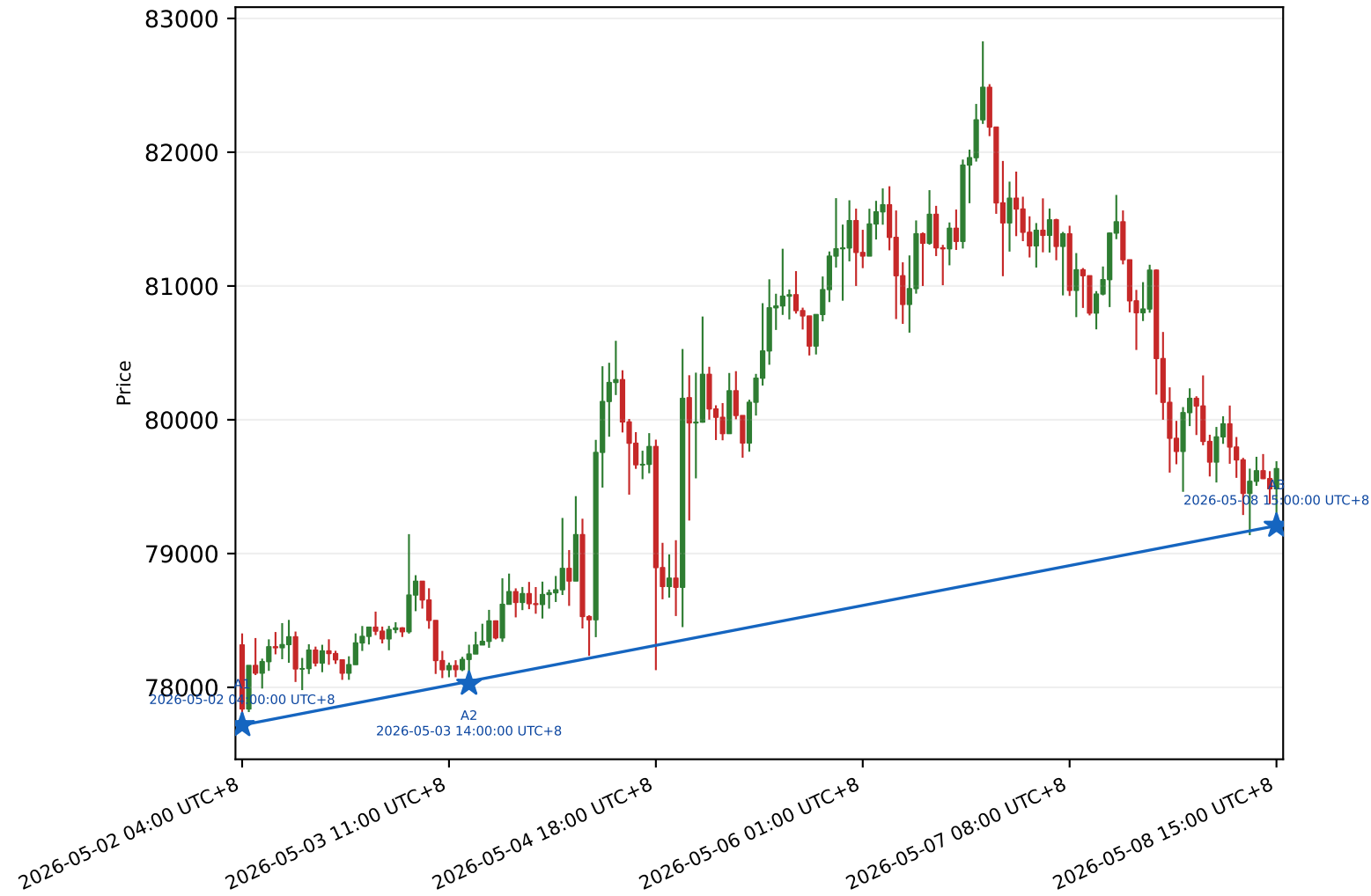
BTC 1h | PATTERN_003 Three Point Trendline Support rule=strict_three_point_slope_support | score=99.58
