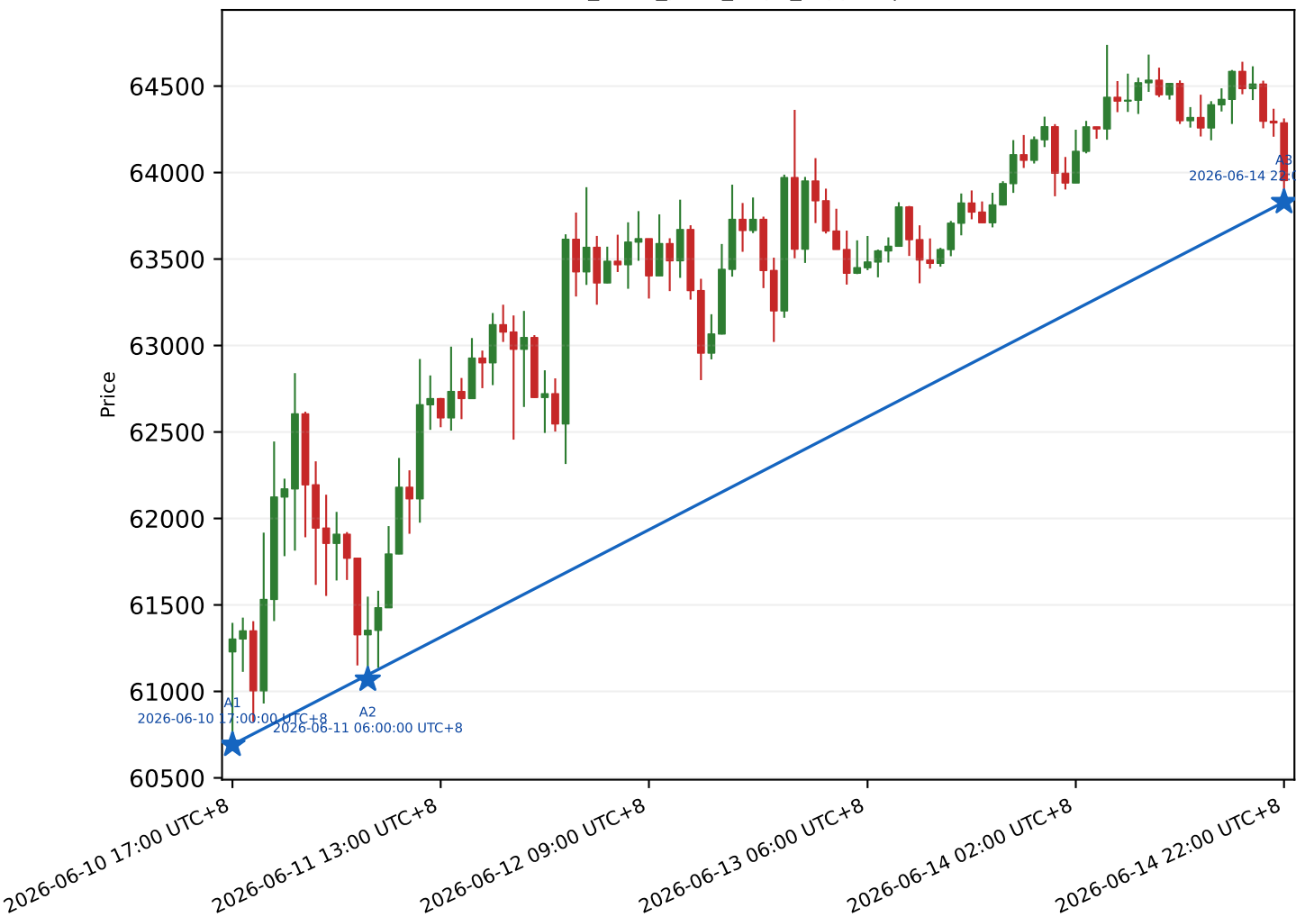
BTC 1h | PATTERN_003 Three Point Trendline Support rule=strict_three_point_slope_support | score=98.99
