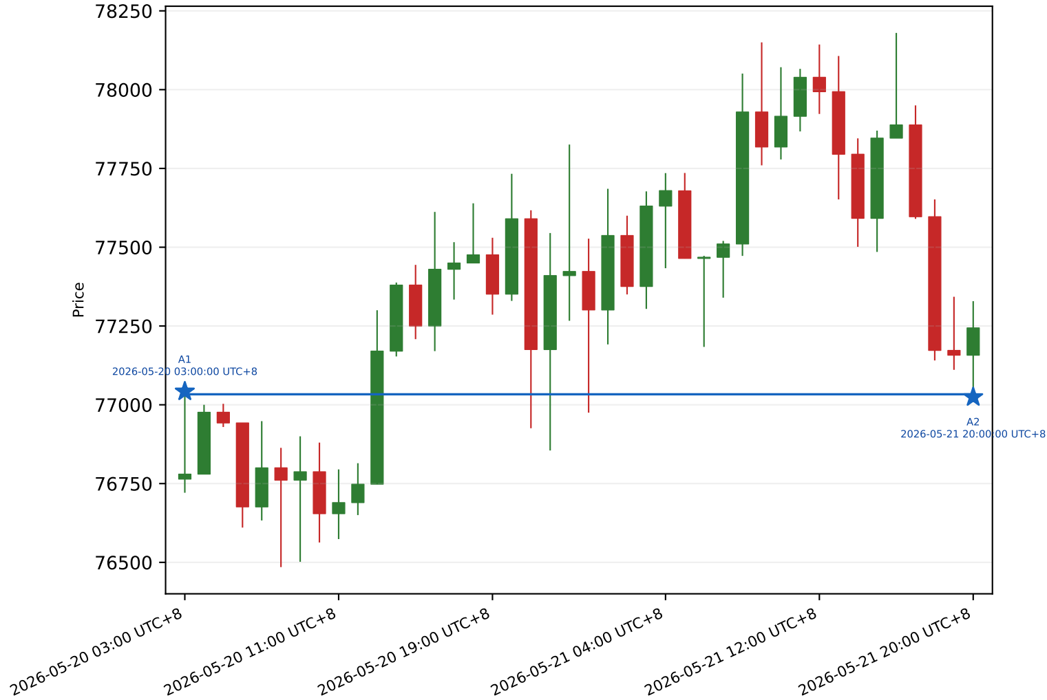
BTC 1h | PATTERN_004 Horizontal Support rule=breakout_retest | score=89.69
