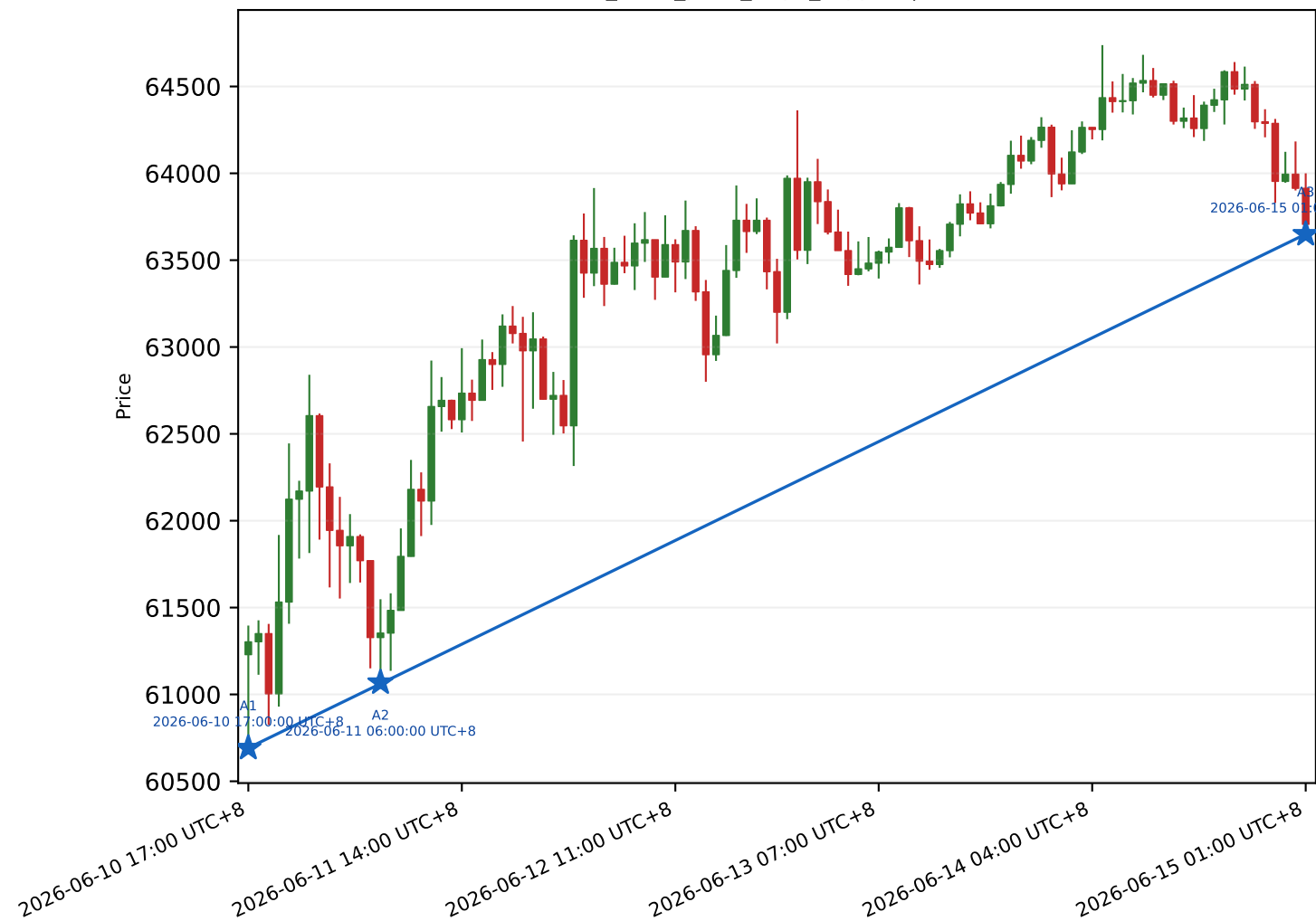
BTC 1h | PATTERN_003 Three Point Trendline Support rule=strict_three_point_slope_support | score=99.75
