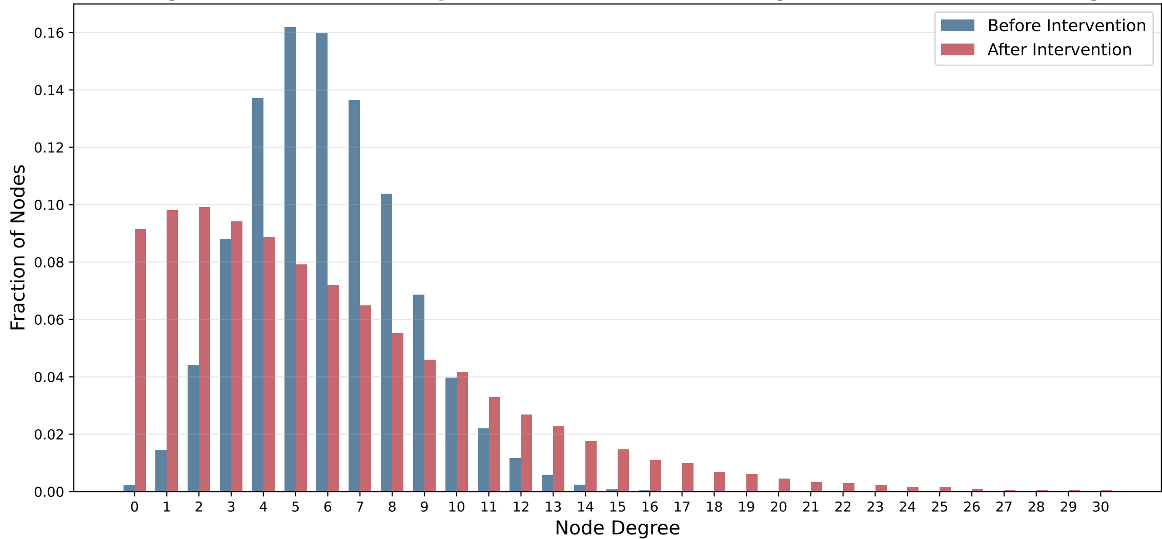
Degree Distribution Comparison: Before vs After Degree-Preferential Rewiring
