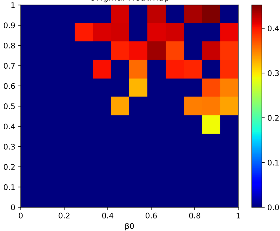
Original Heatmap
