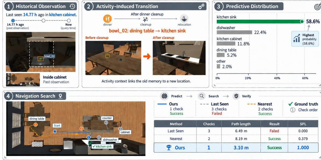
Figure 5: P4D-Bench case study from historical observation to belief-guided navigation. Predictive search reaches the activity-induced current state in one inspection, while last-seen and nearest-first search follow less efficient candidate orders.
