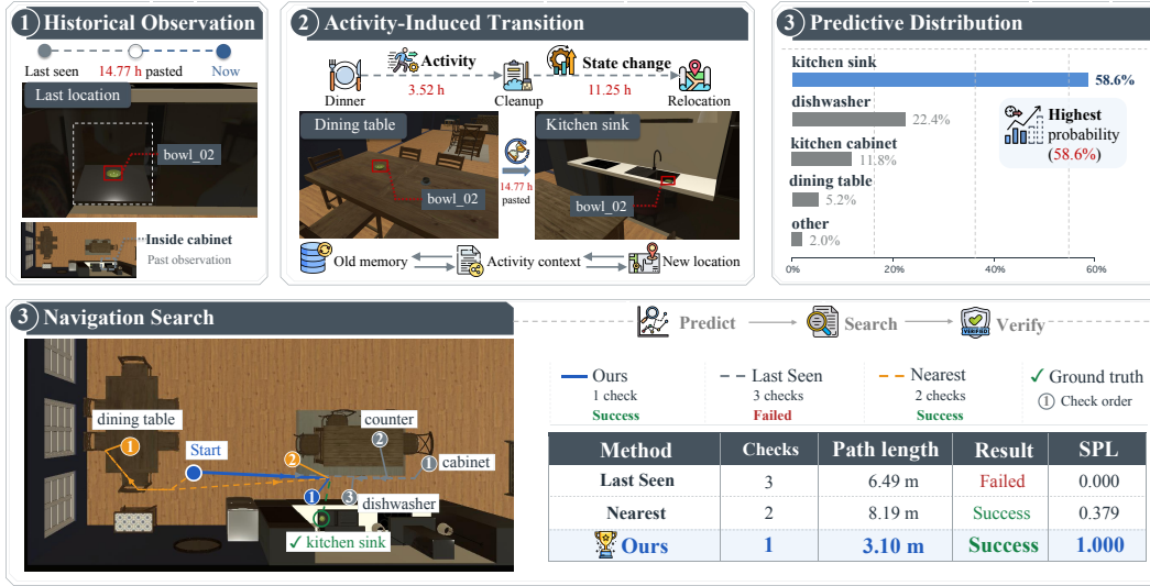
Figure 4: P4D-Bench case study comparing predictive, last-seen, and nearest-first search.
