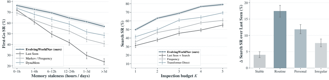
Figure 8: Predictive-memory diagnostics across temporal staleness, inspection budgets, and hidden mobility types.
