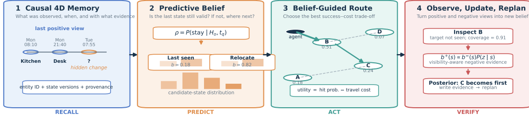
Figure 2: Predictive-navigation core of DR-AGENTOS. A causal 4D memory is propagated to the query time as a structured current-state belief, which the agent uses to plan, inspect, update its evidence, and replan.
