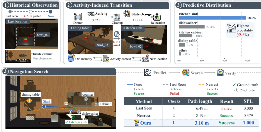
Figure 4: P4D-Bench case study comparing predictive, last-seen, and nearest-first search.
