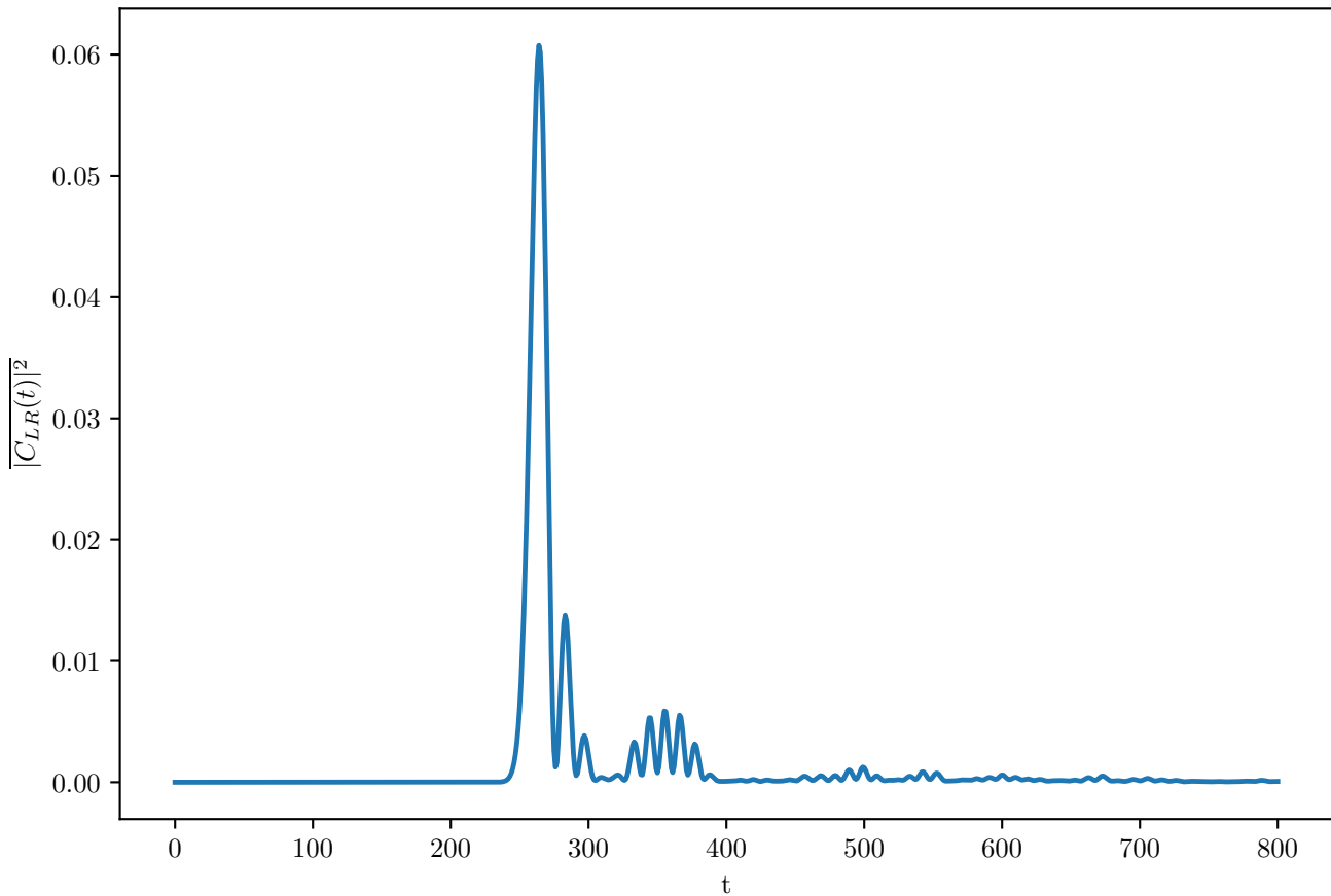
Disorder-averaged corner-to-corner correlator
