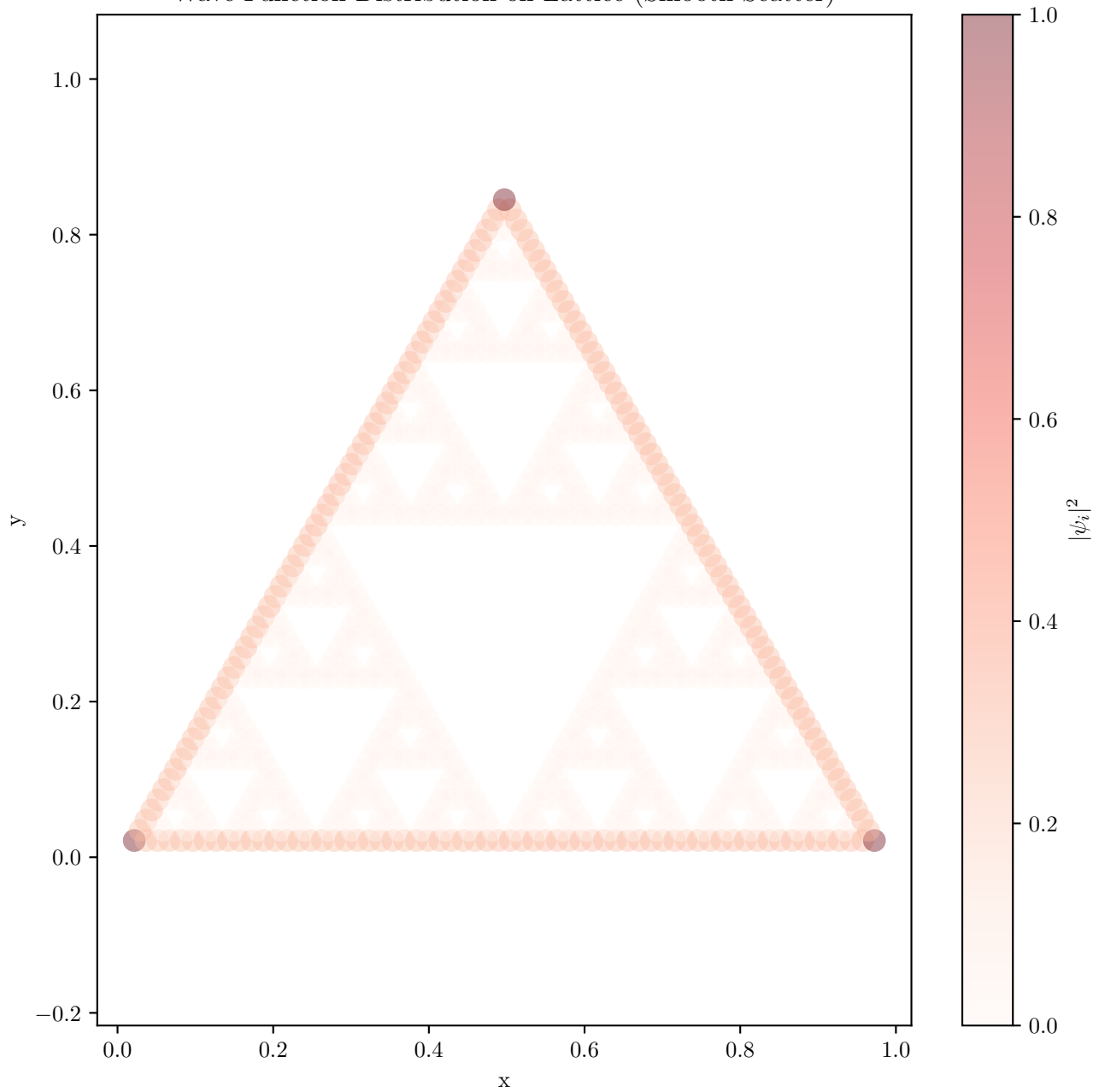
Wave Function Distribution on Lattice (Smooth Scatter)
