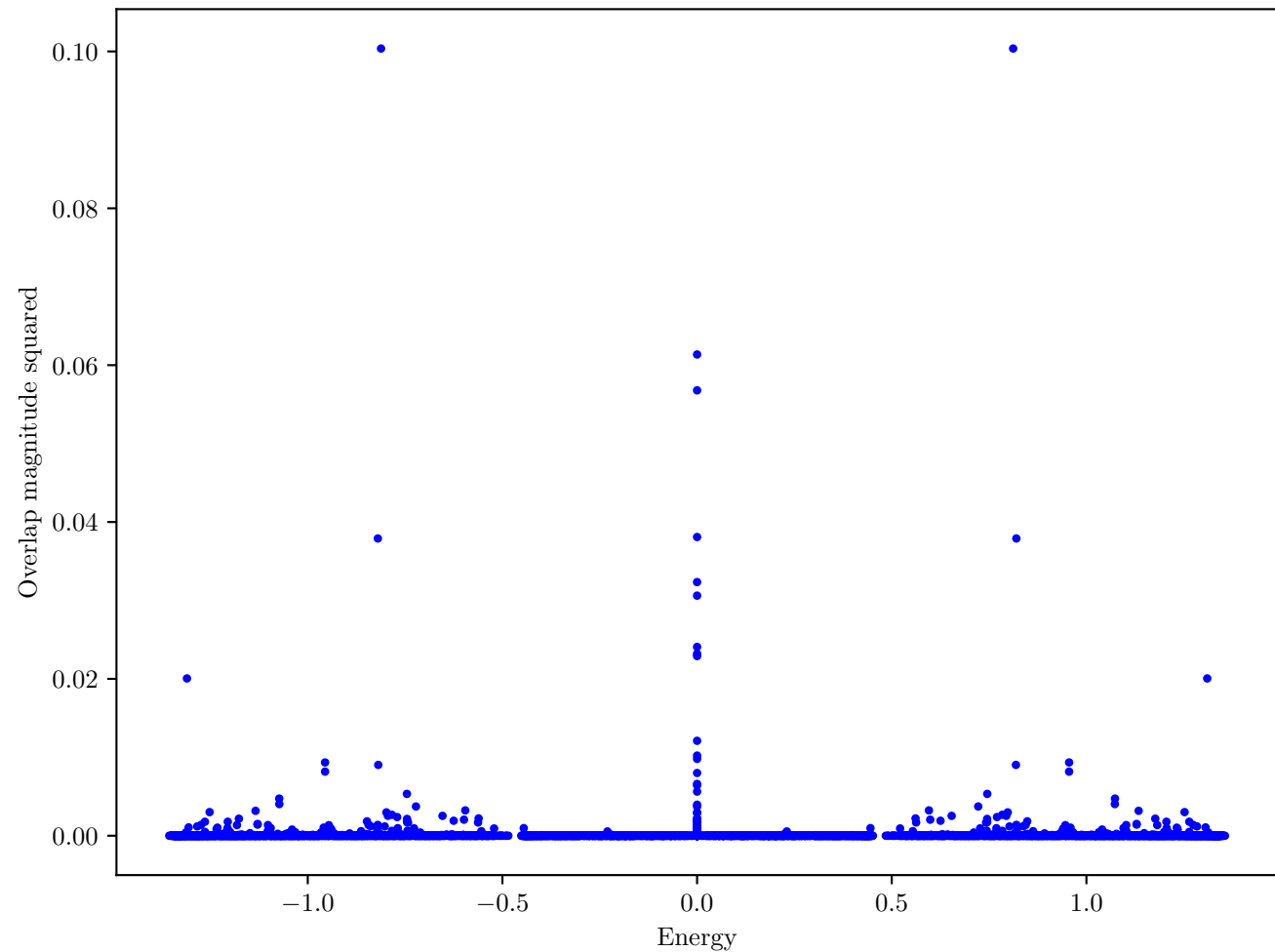
Overlap of State with Eigenstates vs. Energy
