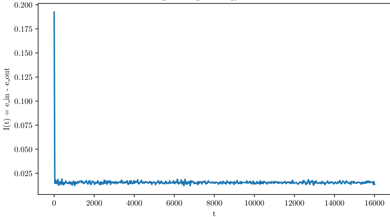
Gauge-averaged energy imbalance
