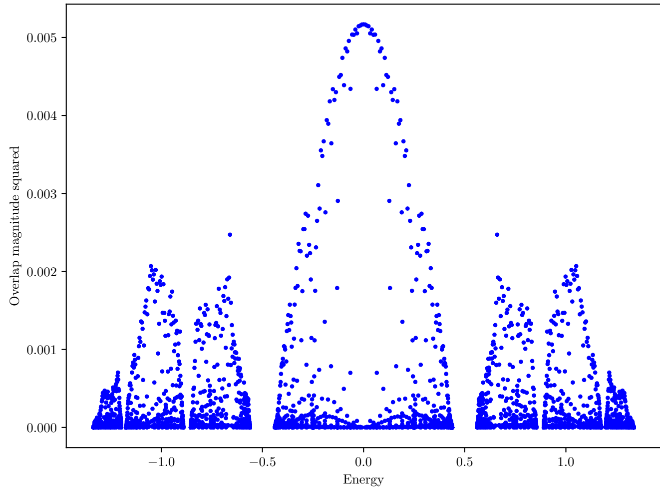
Overlap of State with Eigenstates vs. Energy
