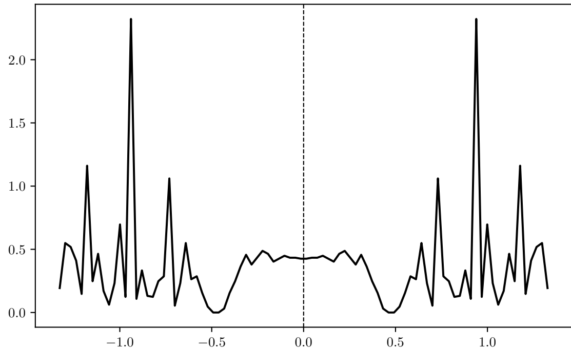
Density of states
