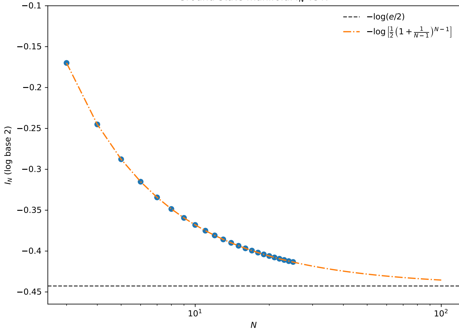
Ground-state manifold: I_N vs N
