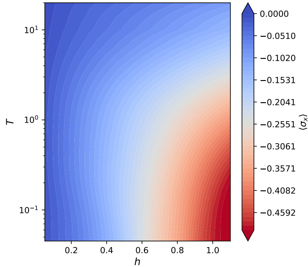
\langle \sigma_x \rangle vs (h, T)
