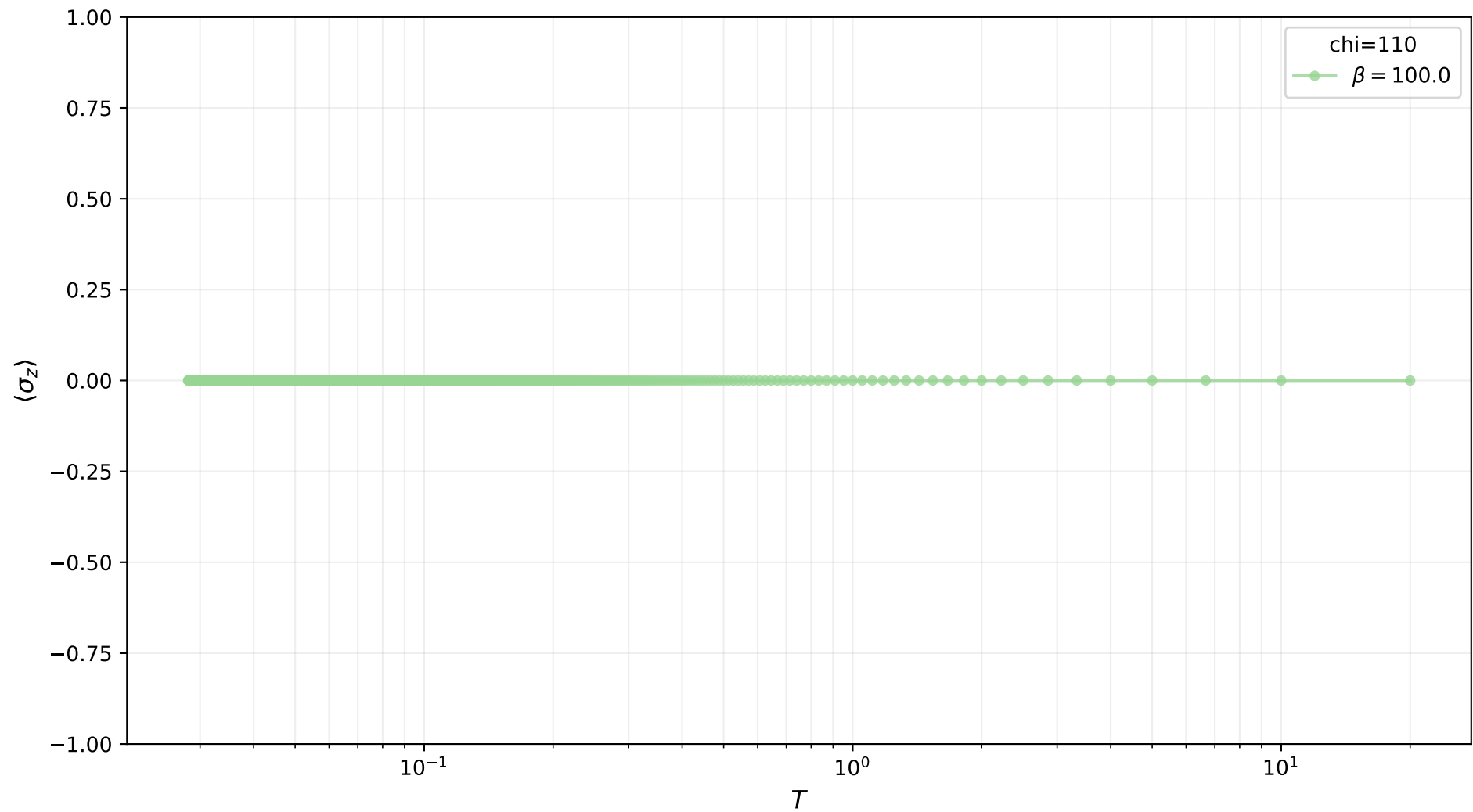
\langle \sigma_z \rangle vs T (chi=110)
