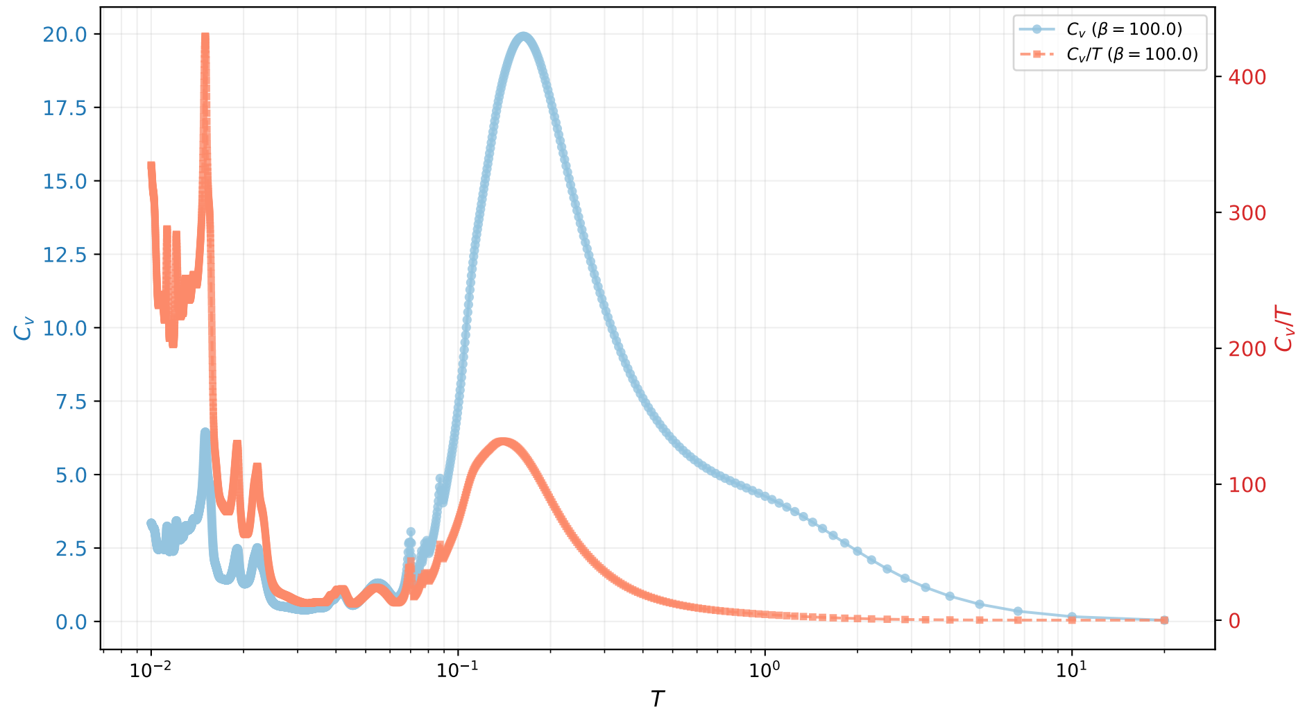
C_v and C_v/T vs T ( \chi=110 )
