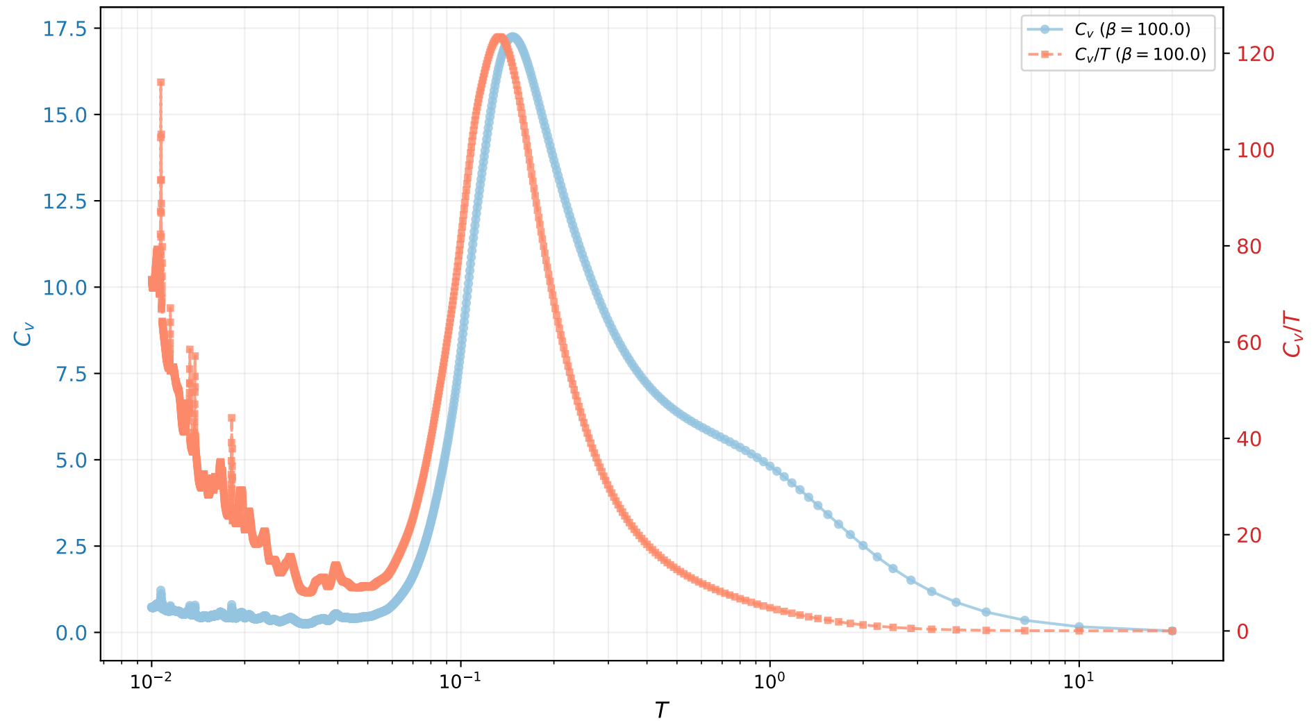
C_v and C_v/T vs T ( \chi=270 )
