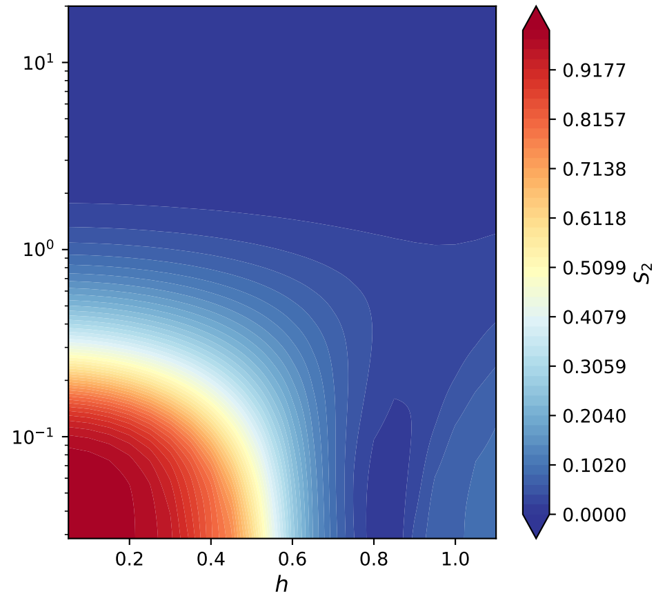
S_2 vs (h, T)
