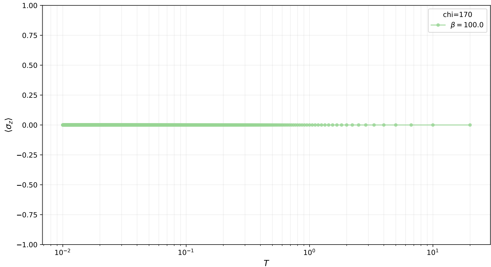
\langle \sigma_z \rangle vs T (chi=170)
