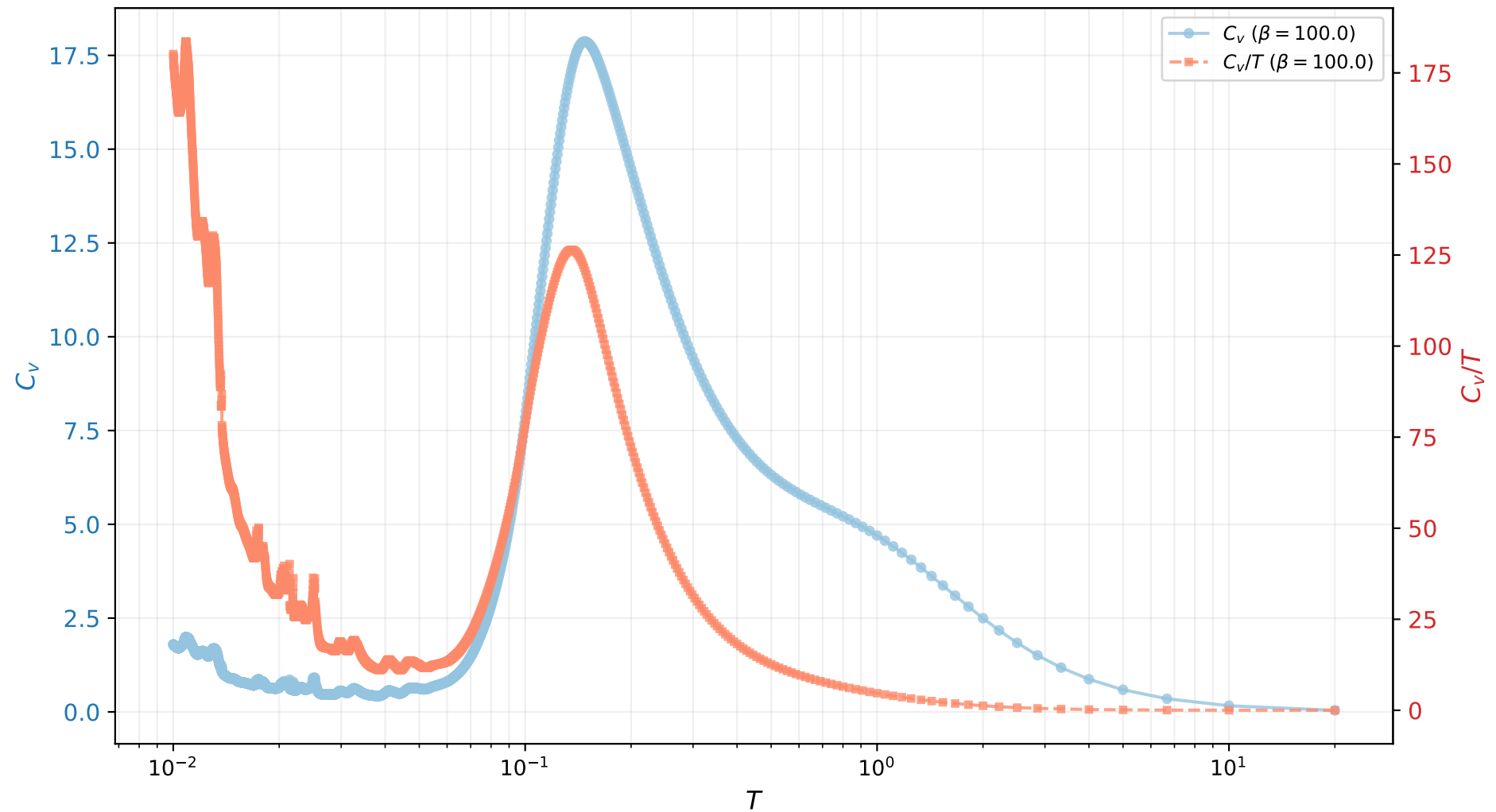
C_v and C_v/T vs T ( \chi=230 )
