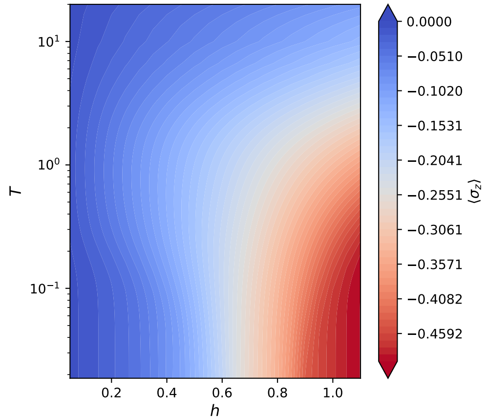
\langle \sigma_z \rangle vs (h, T)
