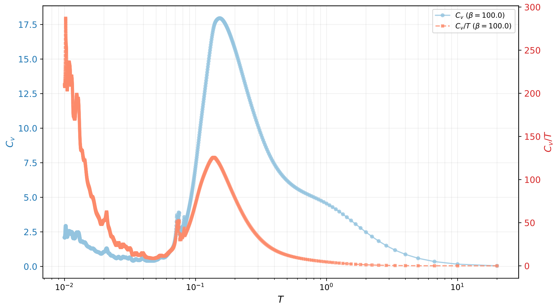
C_v and C_v/T vs T ( \chi=190 )
