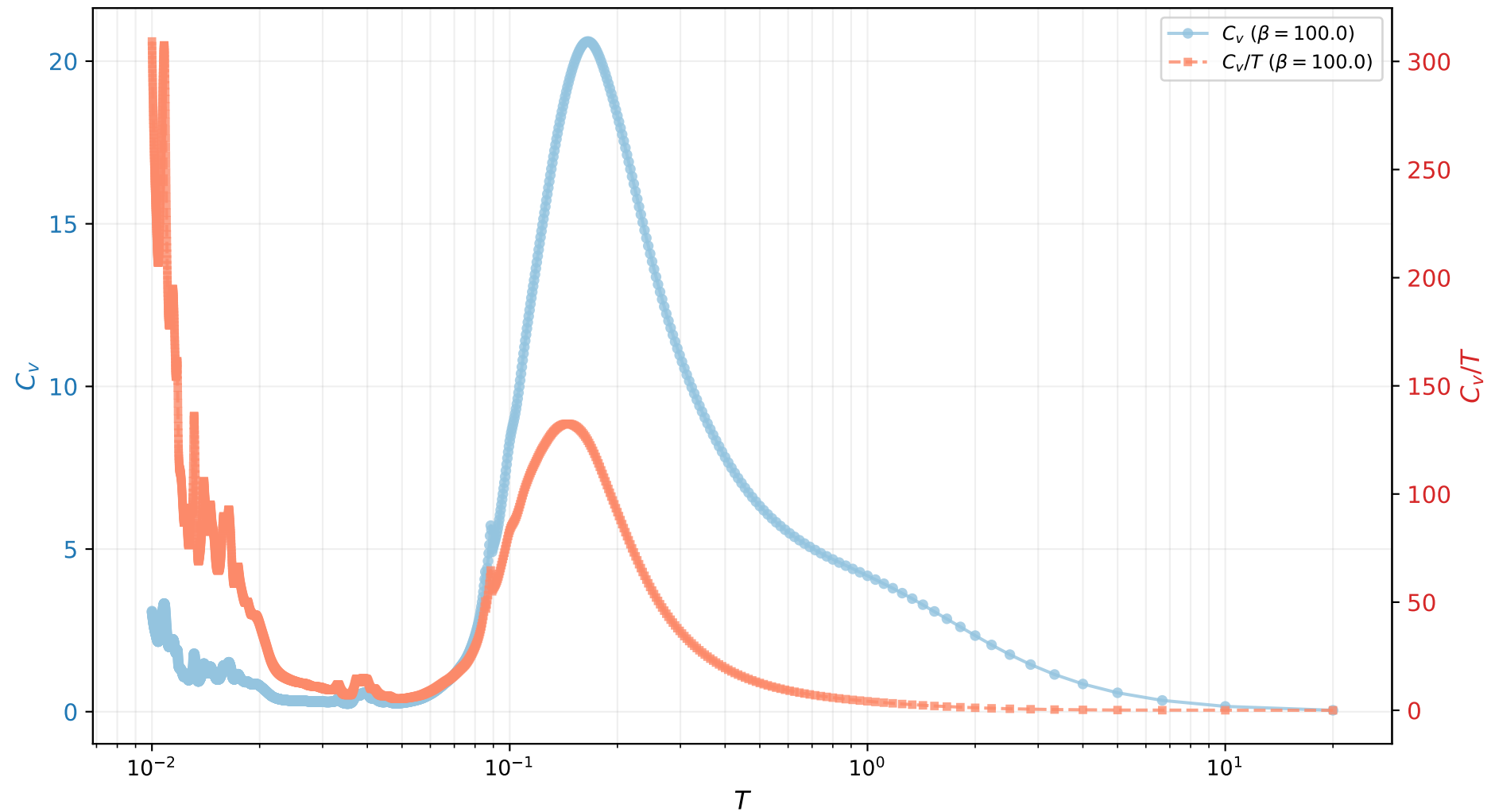
C_V and C_V/T vs T ( \chi=90 )
