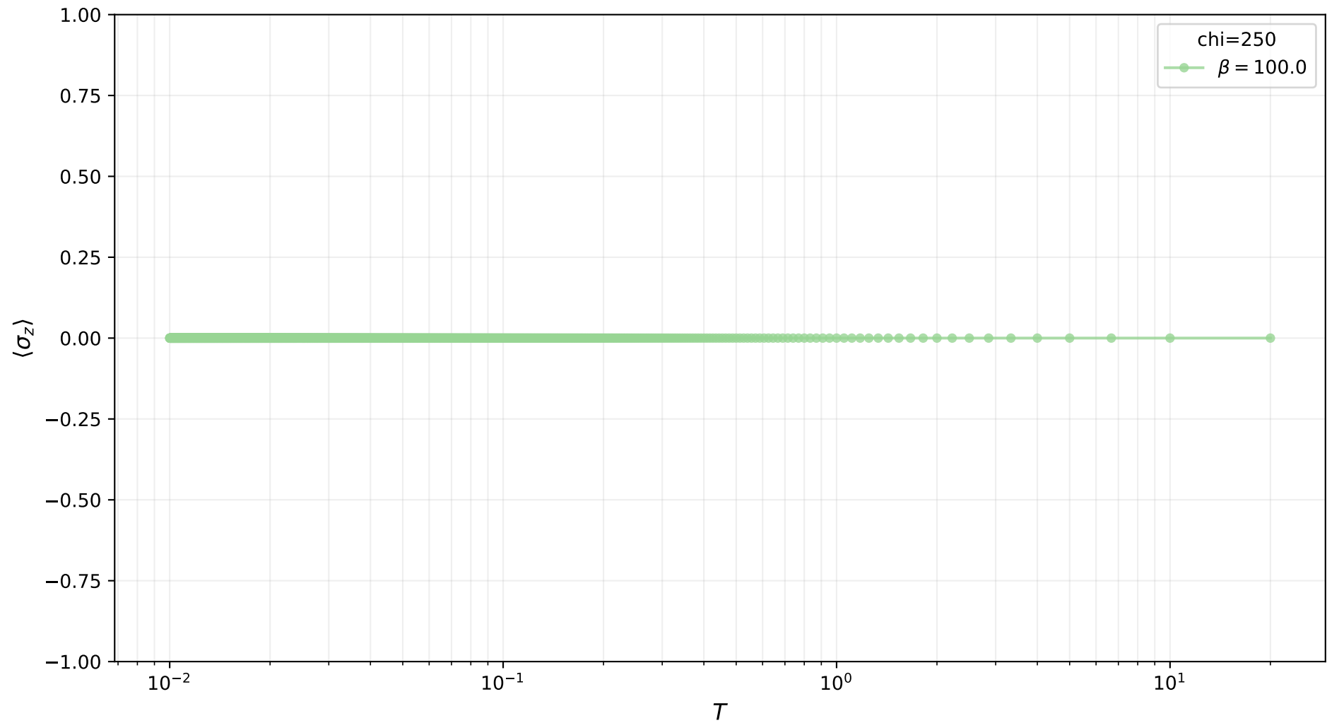
\langle \sigma_z \rangle vs T (chi=250)
