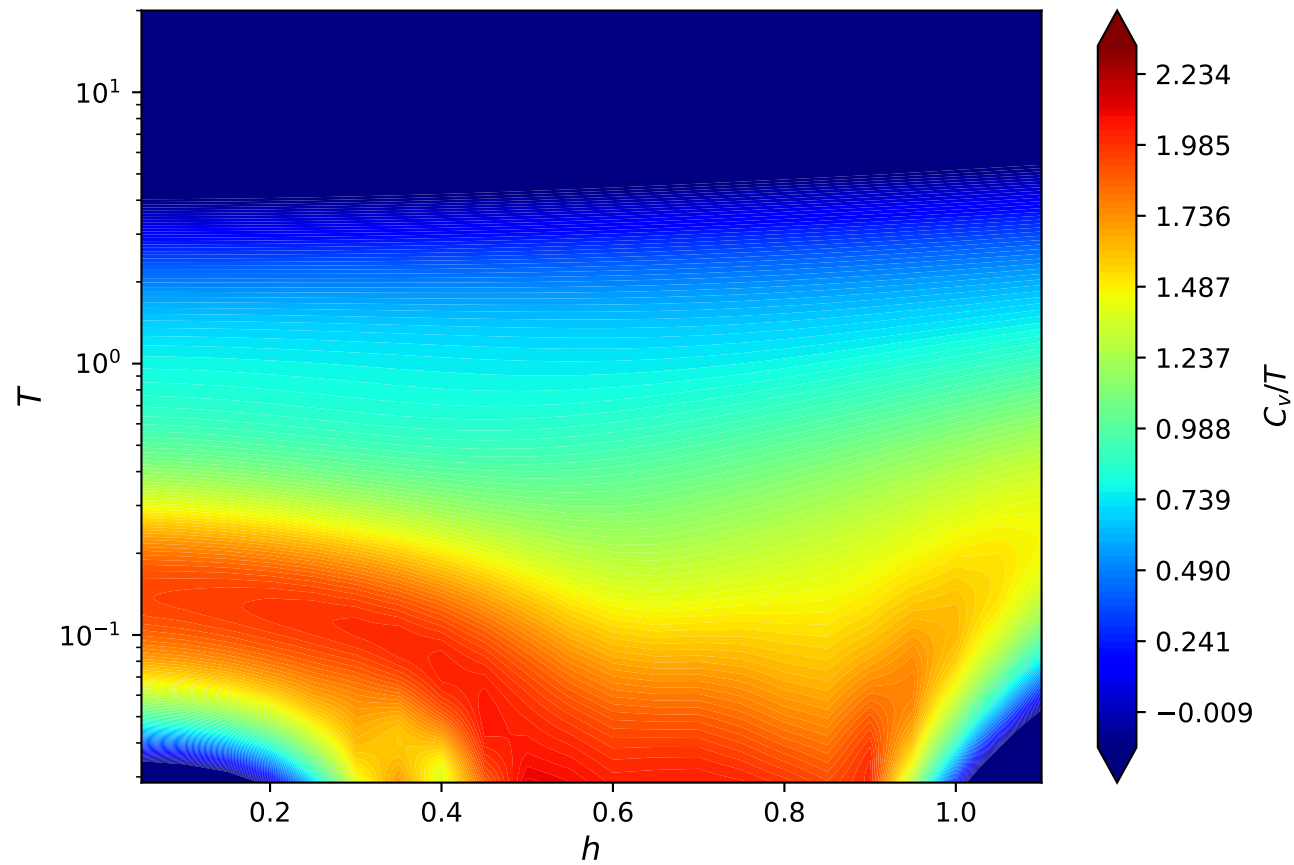
C_v/T vs (h, T)
