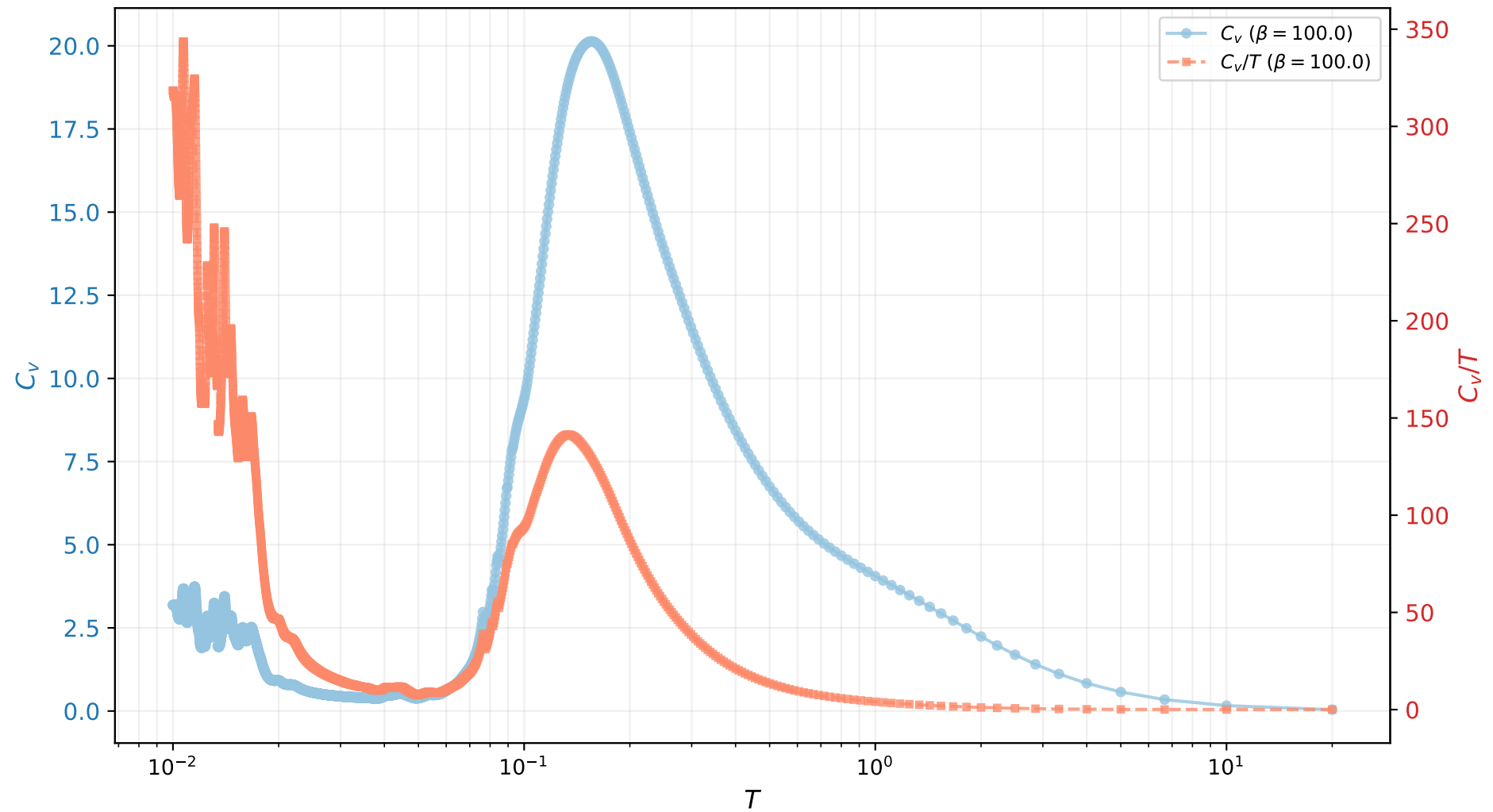
C_v and C_v/T vs T ( \chi=70 )
