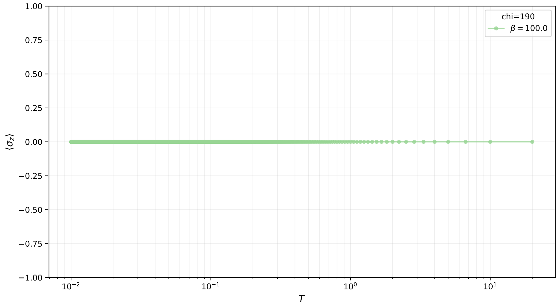
\langle \sigma_z \rangle vs T (chi=190)
