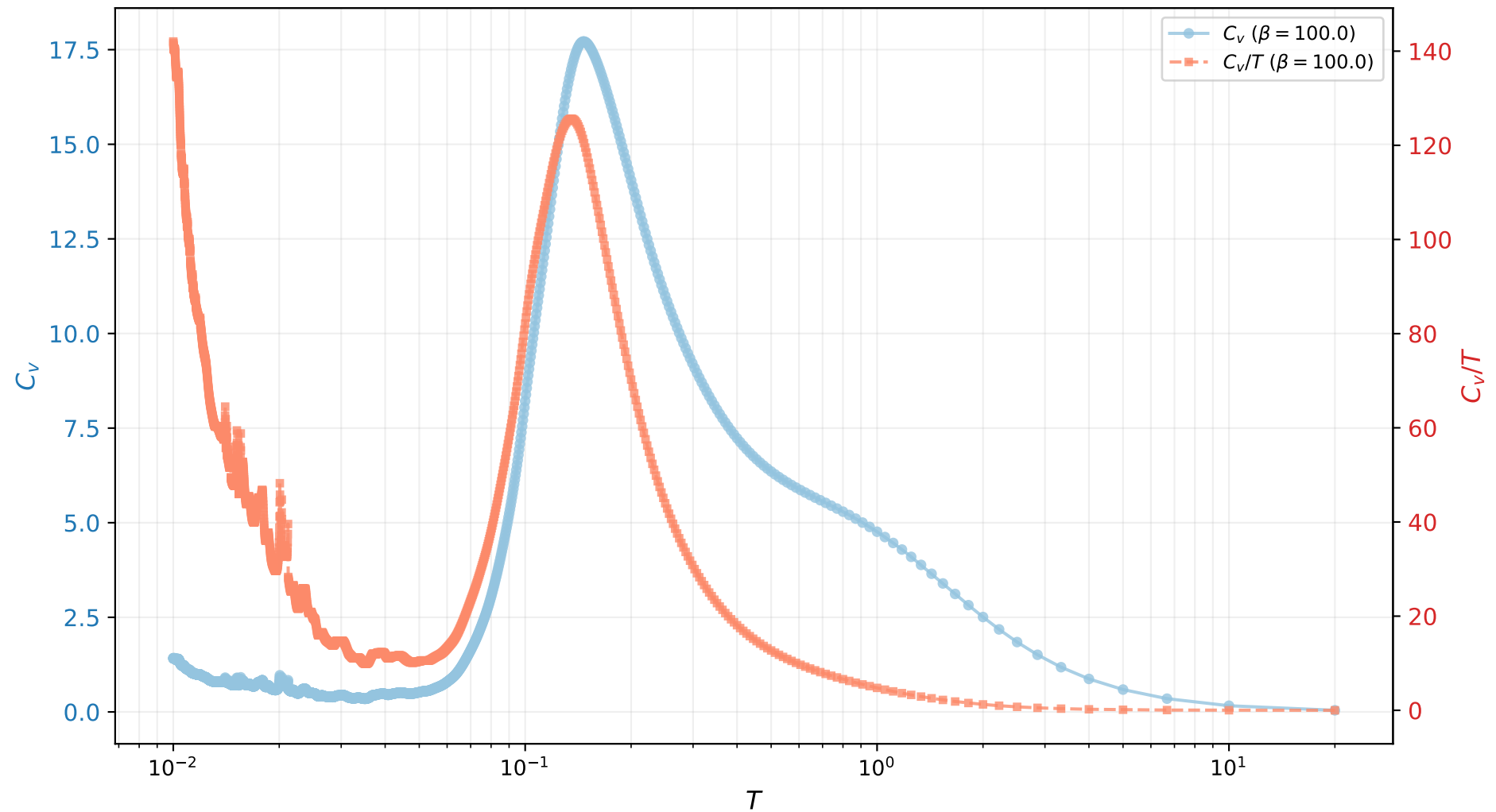
C_v and C_v/T vs T ( \chi=250 )
