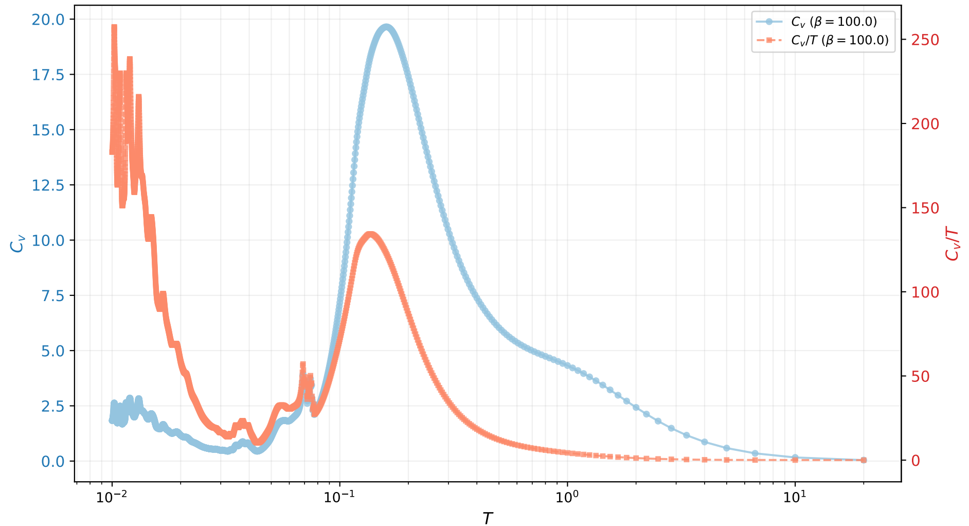
C_v and C_v/T vs T ( \chi=130 )
