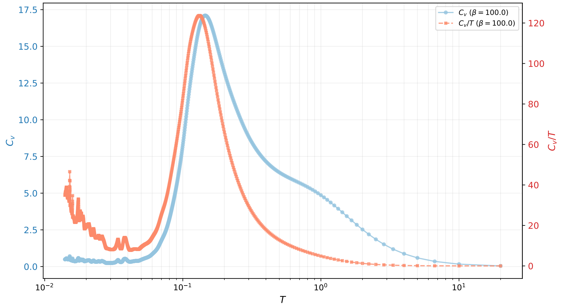
C_v and C_v/T vs T ( \chi=290 )
