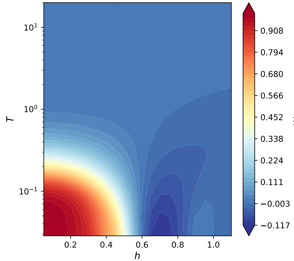
W_p vs (h, T)
