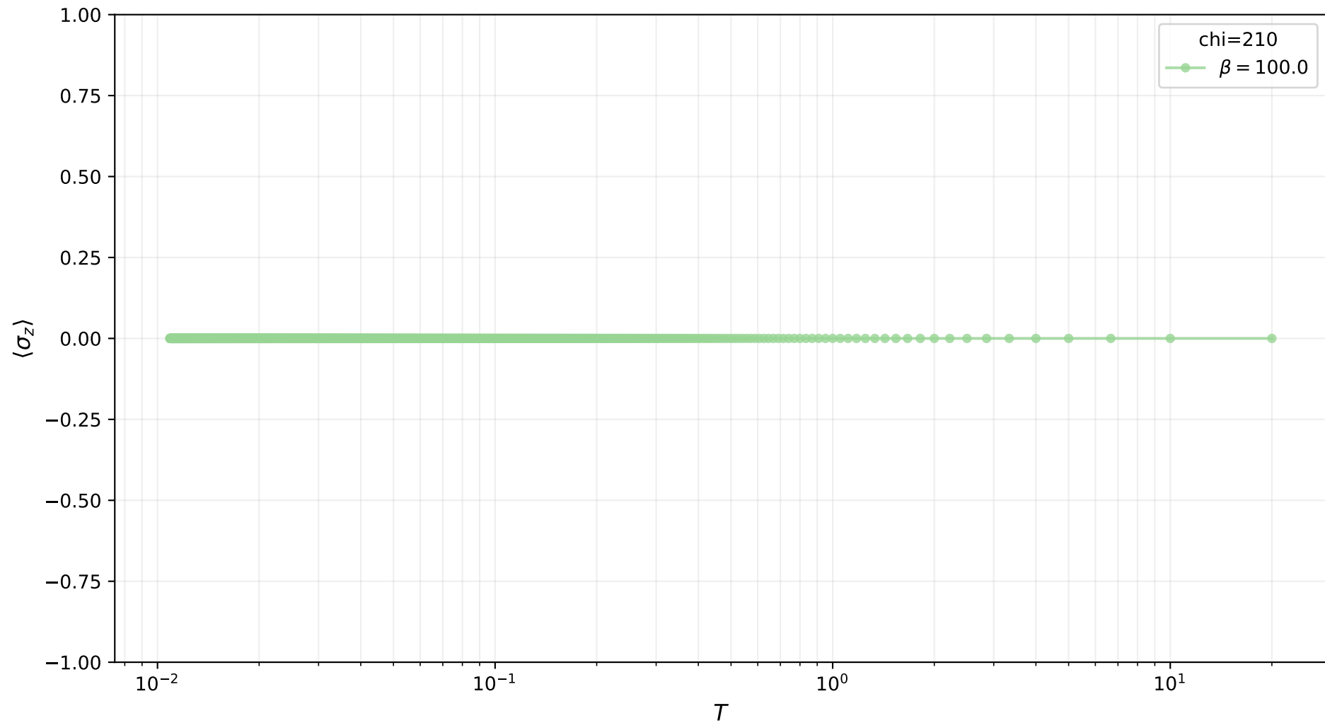
\langle \sigma_z \rangle vs T (chi=210)
