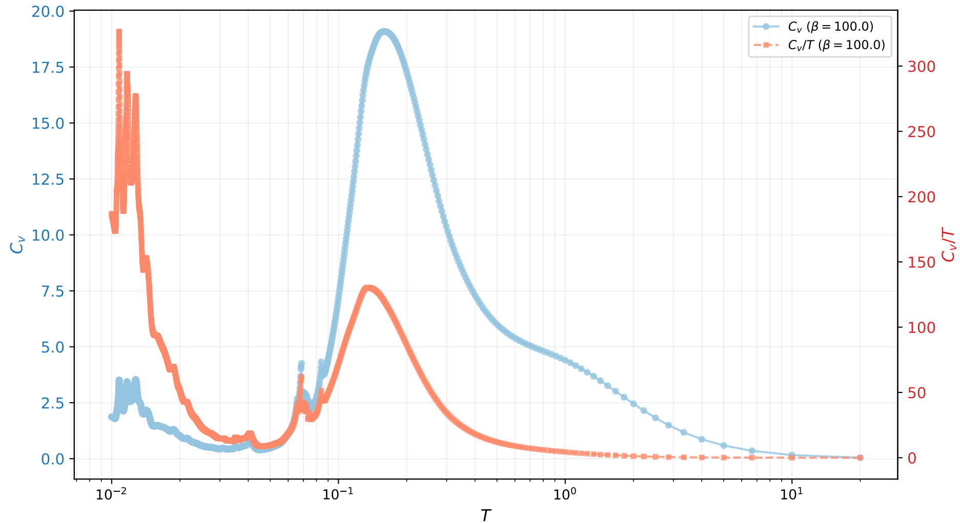
C_v and C_v/T vs T ( \chi=150 )
