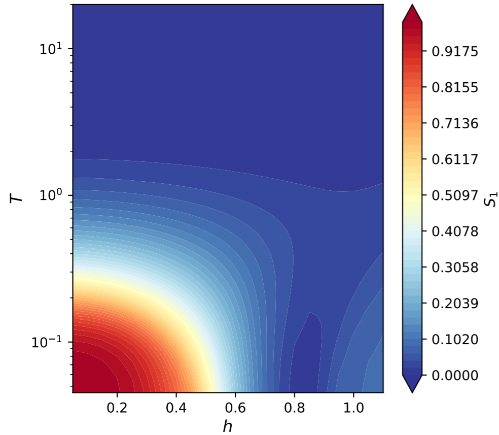
S_1 vs (h, T)
