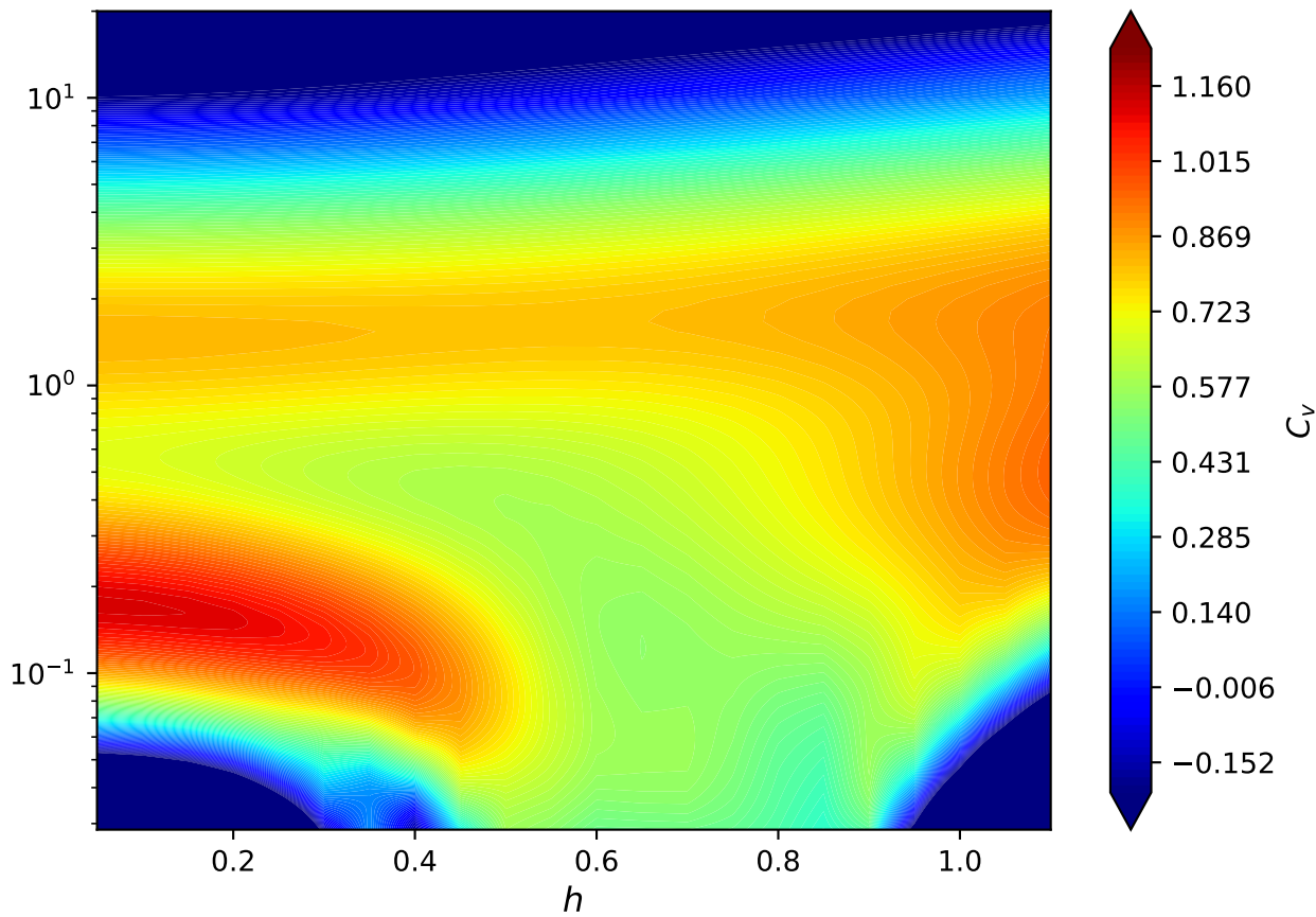
C_v vs (h, T)
