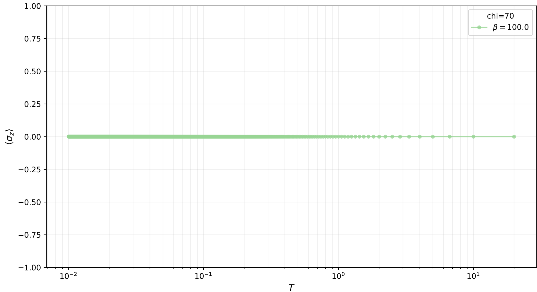
\langle \sigma_z \rangle vs T (chi=70)
