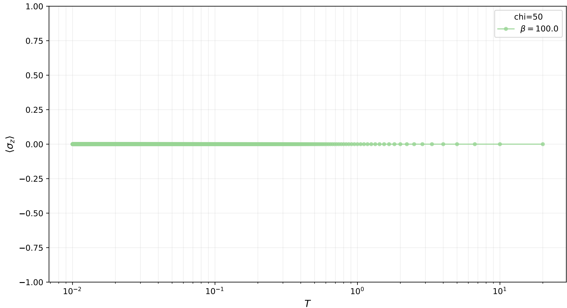
\langle \sigma_z \rangle vs T (chi=50)
