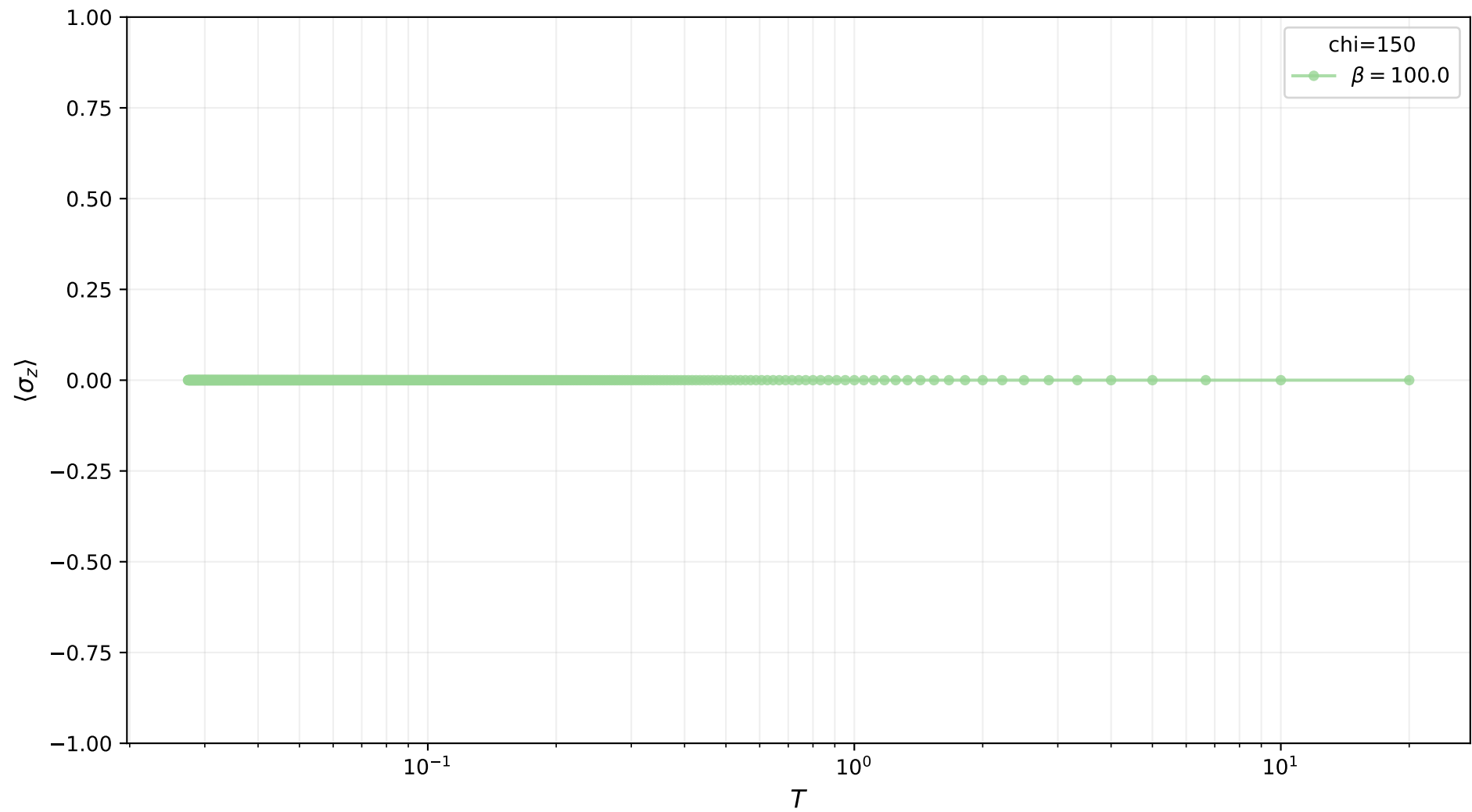
\langle \sigma_z \rangle vs T (chi=150)
