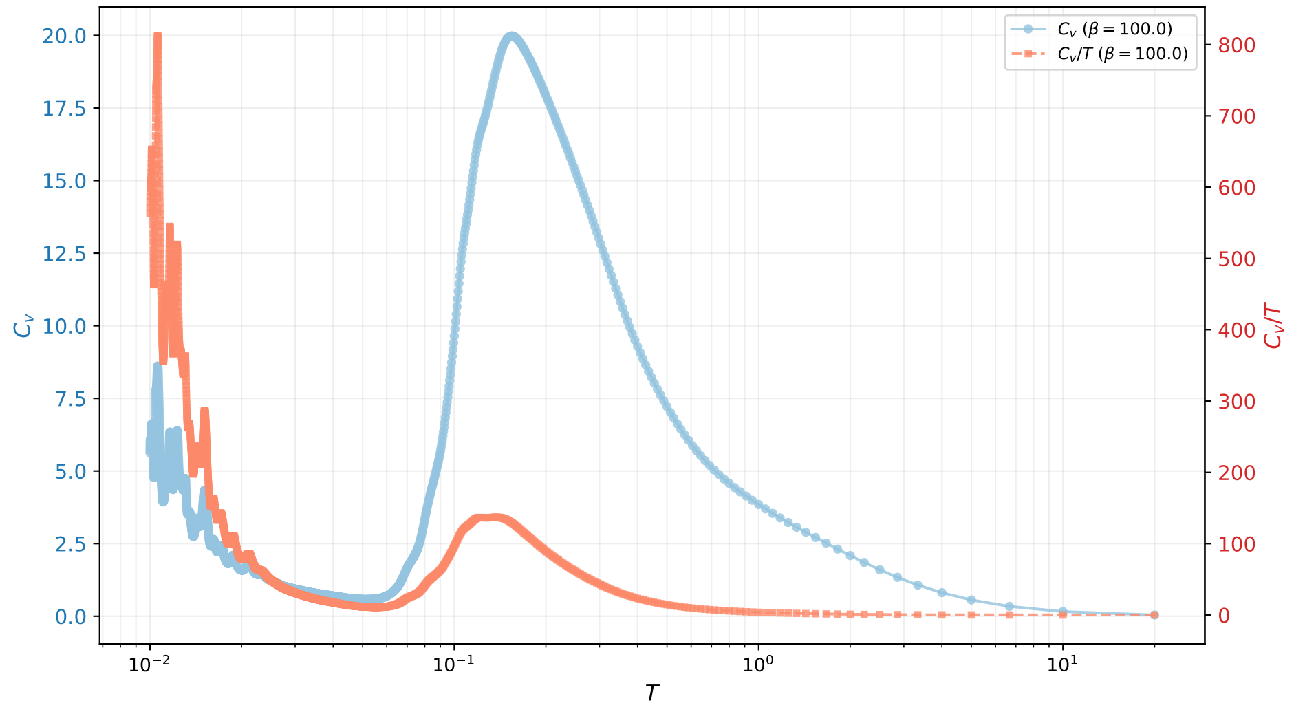
C_v and C_v/T vs T ( \chi=50 )
