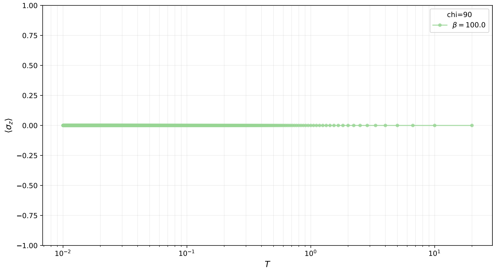
\langle \sigma_z \rangle vs T (chi=90)
