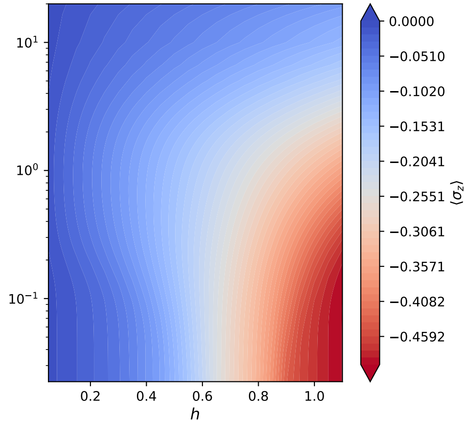
\langle \sigma_z \rangle vs (h, T)
