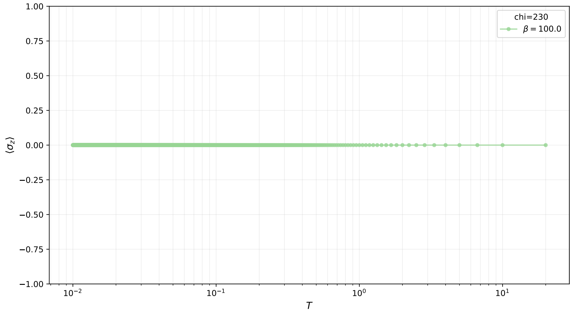
\langle \sigma_z \rangle vs T (chi=230)
