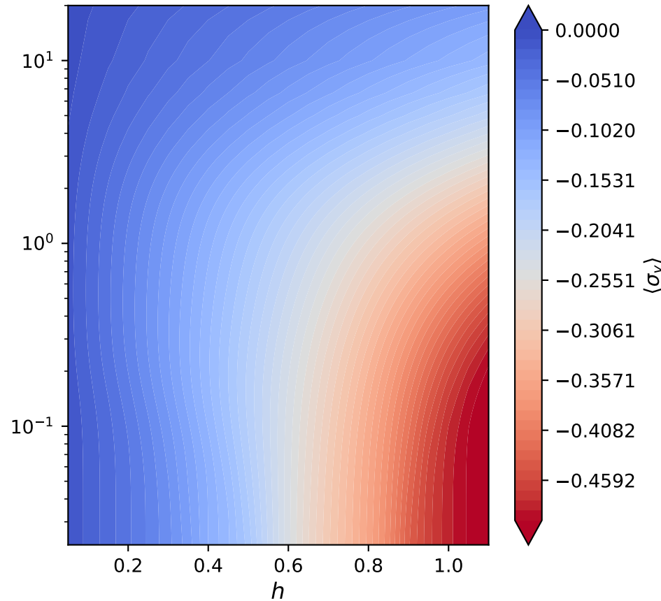
\langle \sigma_y \rangle vs (h, T)
