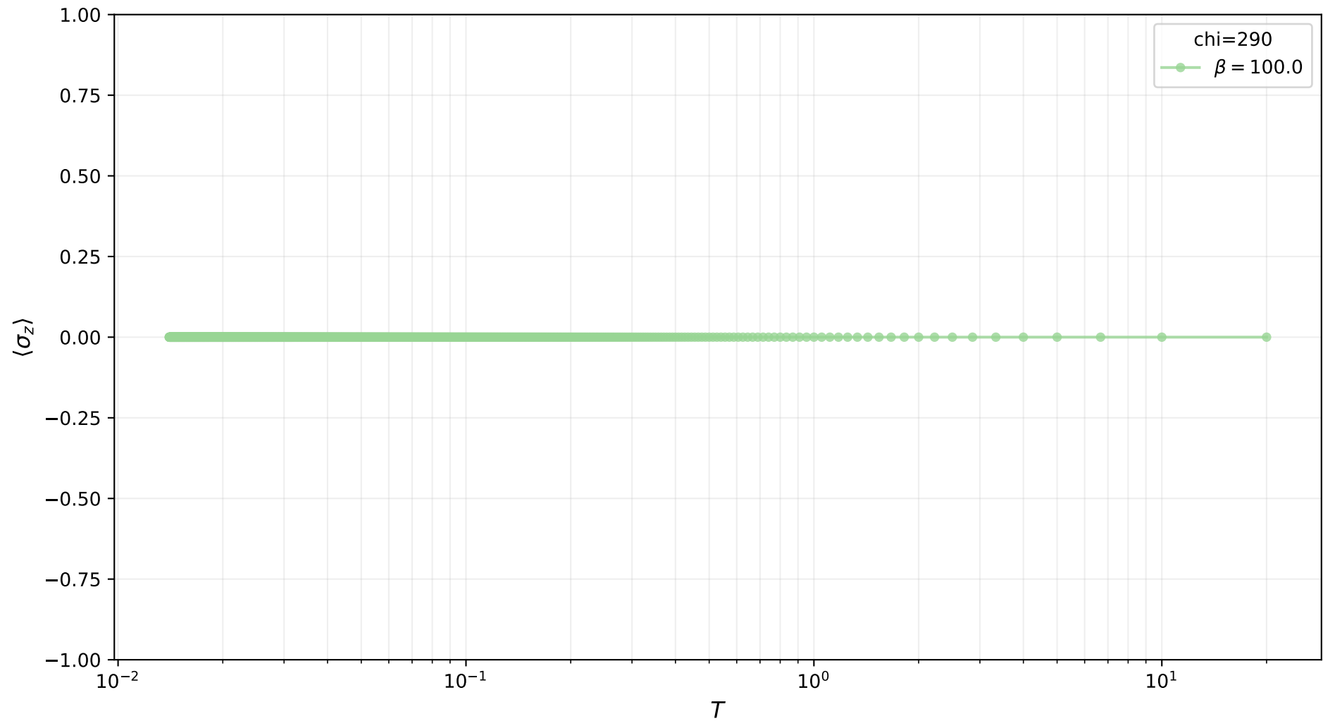
\langle \sigma_z \rangle vs T (chi=290)
