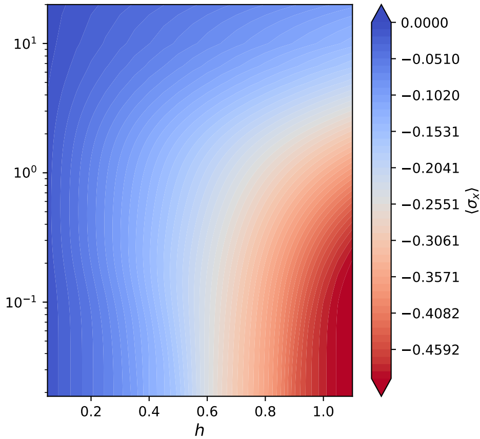
\langle \sigma_x \rangle vs (h, T)
