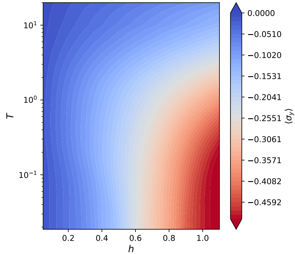
\langle \sigma_y \rangle vs (h, T)
