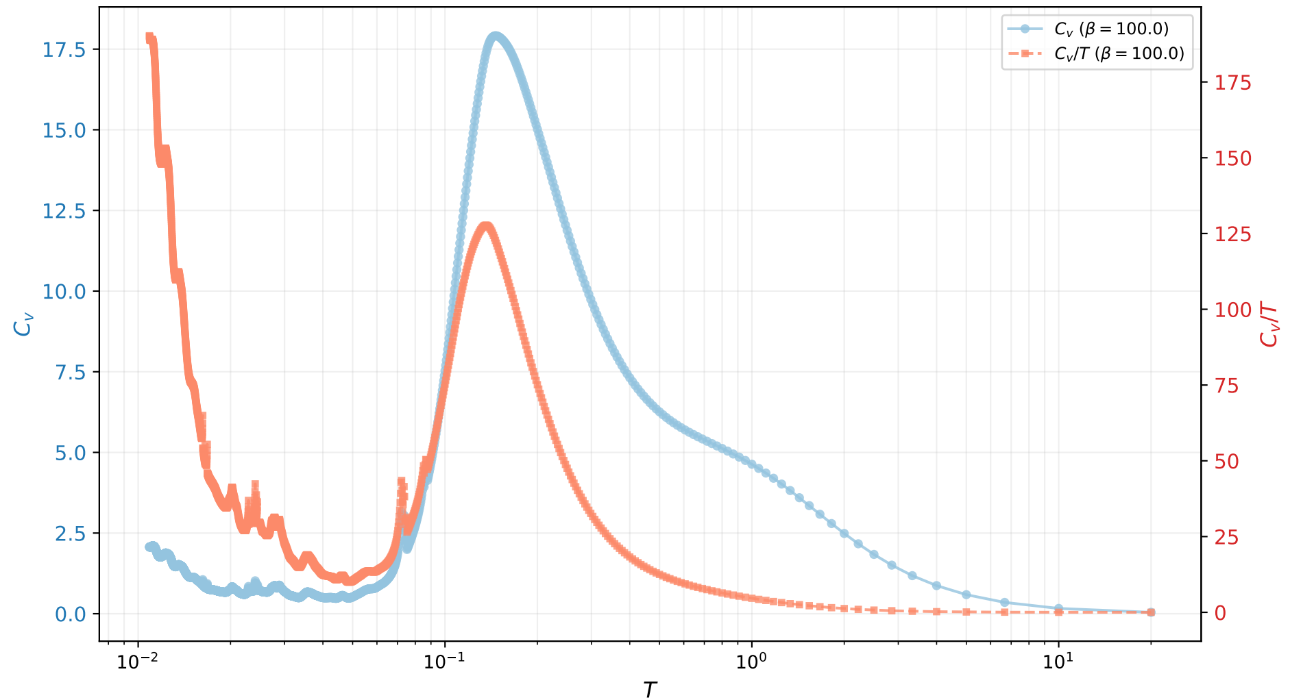
C_v and C_v/T vs T ( \chi=210 )
