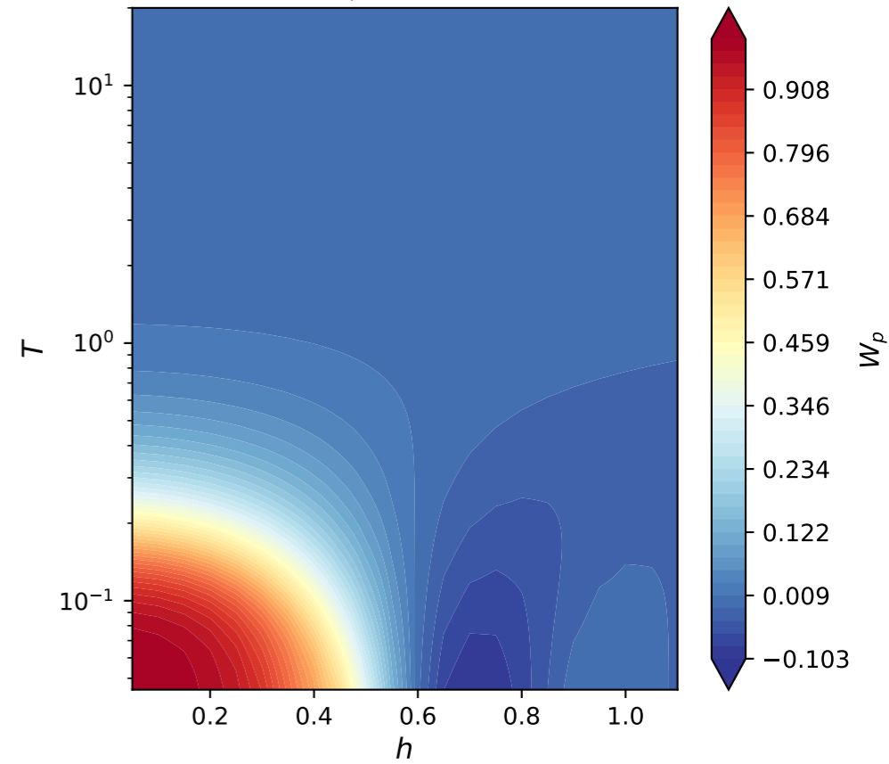
W_p vs (h, T)
