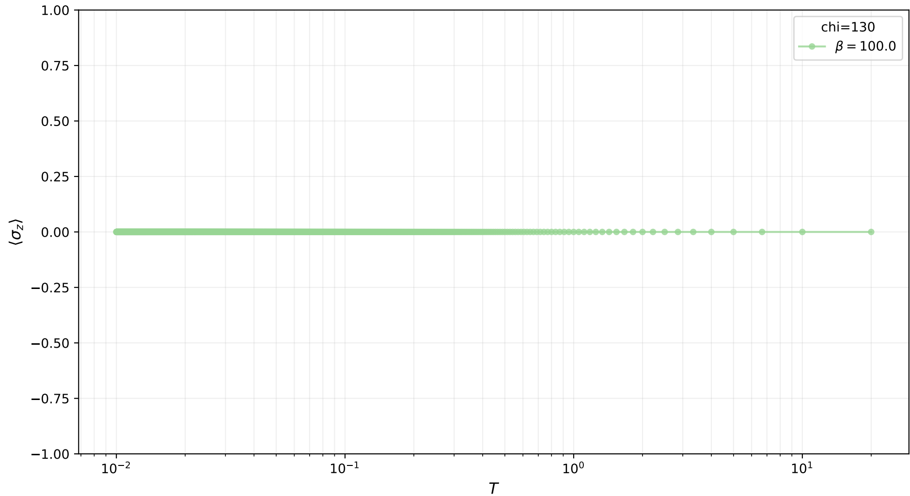
\langle \sigma_z \rangle vs T (chi=130)
