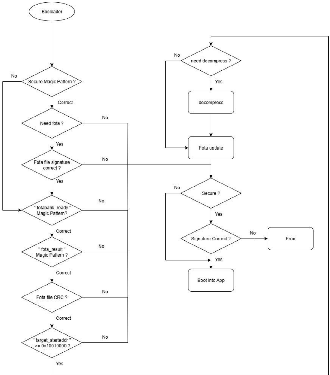
Figure1. Bootloader flow chat
