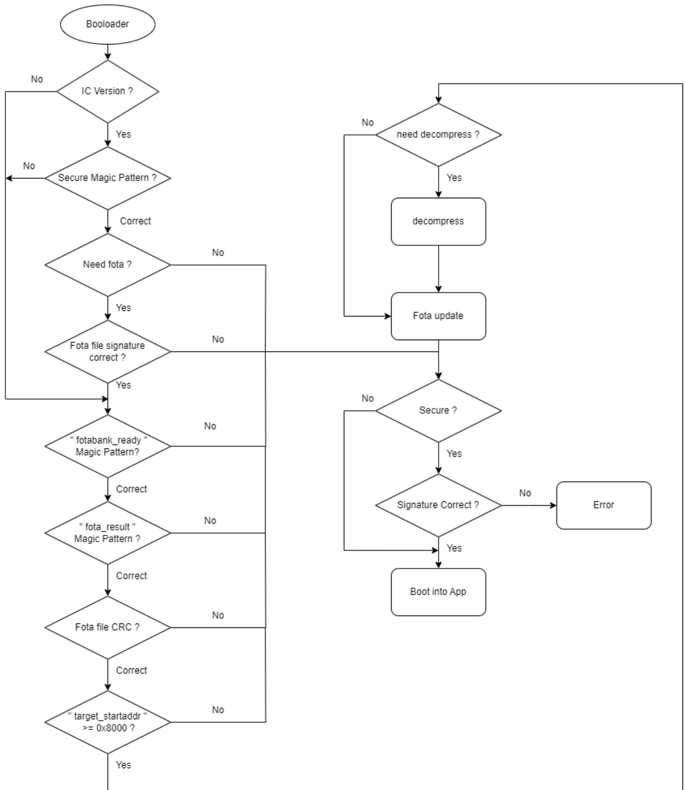
Figure1. Bootloader flow chat
