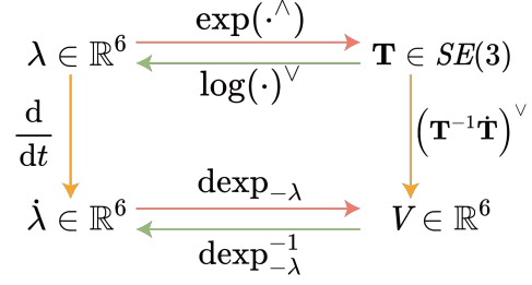
Fig. 1. Transformation between SE(3) and exponential coordinates.
