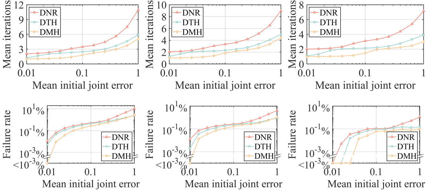
Fig. 11. Simulation #5: Robustness of the DNR, DTH, and DMH methods on various robots. Mean iterations and failure rate for UR5 (left), FANUC M-710iC (middle), KUKA LBR IIWA 14R820 (right) robots.
