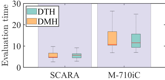
Fig. 9. Simulation #4: Evaluation time of the DTH and DMH methods on the FANUC M-710iC and SCARA robots (in \mu\text{s} ).
