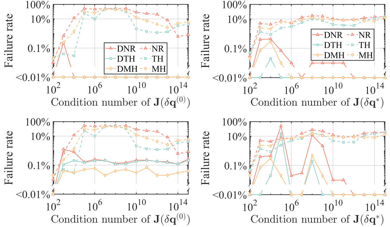
Fig. 12. Simulation #6: Reliability of the NR, TH, MH, DNR, DTH, and DMH methods on the UR5 robot. Near-singular points are at the initial and target configurations for \epsilon = 10^{-8} (top) and \epsilon = 10^{-10} (bottom).
