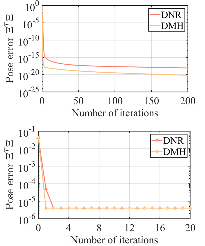
Fig. 7. Simulation #3: Comparison between DMH and DNR on the FANUC M-710iC robot under noise-free scenario (top) and noisy scenario (bottom).
