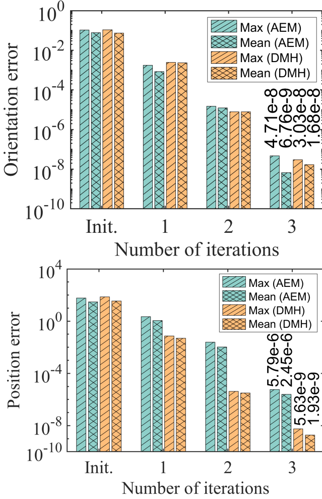
Fig. 4. Simulation #2: Comparison between DMH and AEM on the Motoman HP20D robot, in terms of orientation error (in rad) and position error (in mm).
