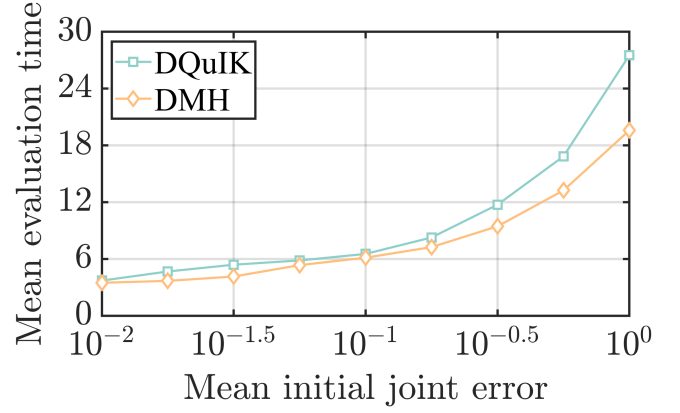
Fig. 10. Simulation #4: Evaluation time of the DQuIK and DMH methods on the UR5 robot (in \mu\text{s} ).
