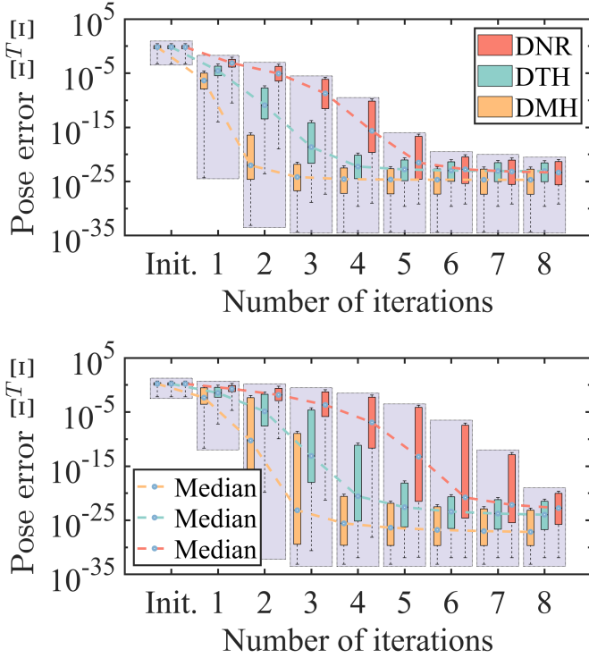
Fig. 8. Simulation #4: Convergence of the DNR, DTH, and DMH methods on the SCARA (top) and FANUC M-710iC (bottom) robots.
