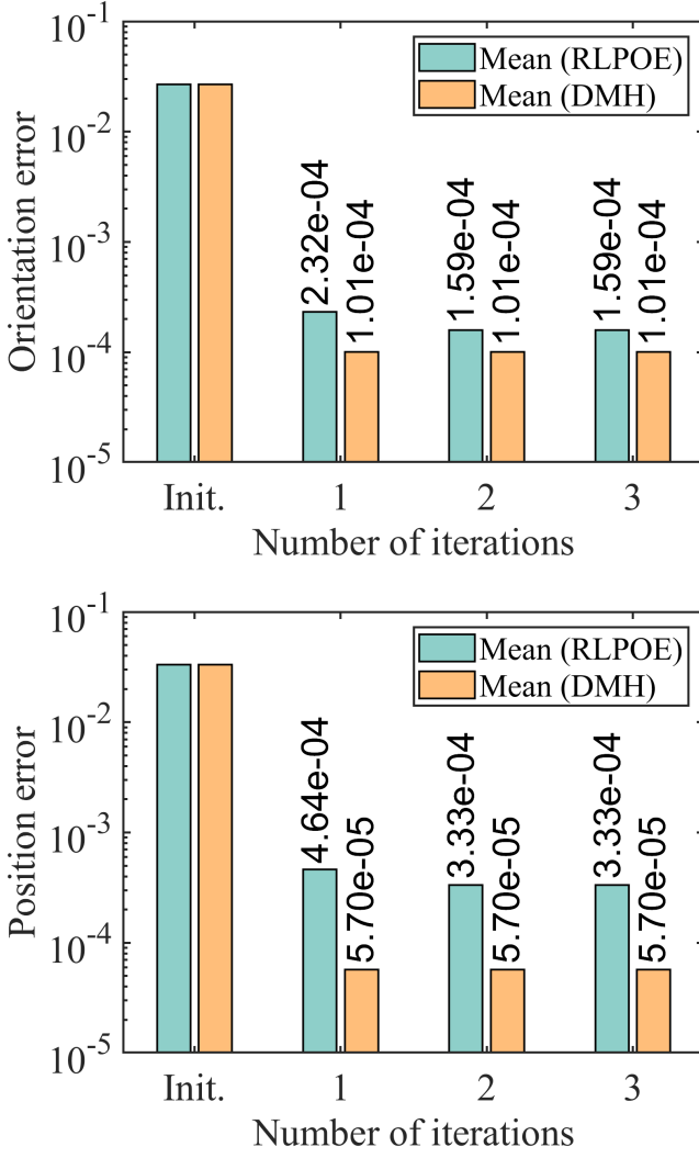
Fig. 6. Simulation #3: Comparison between DMH and RLPOE on the FANUC M-710iC robot under noises, in terms of orientation error (in rad) and position error (in m).
