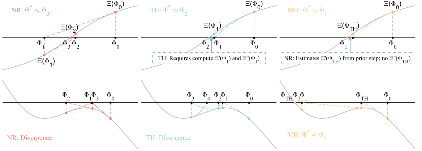
Fig. 3. Graphical illustration of the NR, TH, and MH methods on one-dimensional functions. The MH method achieves the fewest iterations for \Xi(\Phi) = \arctan(\Phi) (top), while the NR and TH methods diverge, with only the MH method converging for \Xi(\Phi) = \sin(\Phi) + 0.5 \cos(3\Phi) - 0.1\Phi (bottom). In the latter case, the \Xi'(\Phi_{TH}) estimated by \Xi''(\Phi_0) has the opposite sign of the true \Xi'(\Phi_{TH}) , which facilitates convergence.
