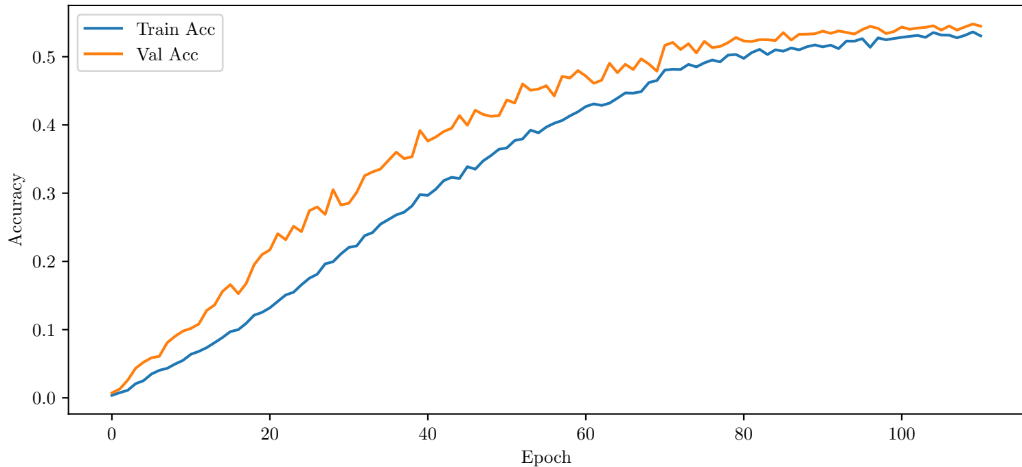
GSL Transformer — Accuracy — d_{\text{model}} = 128 — Augmentation
