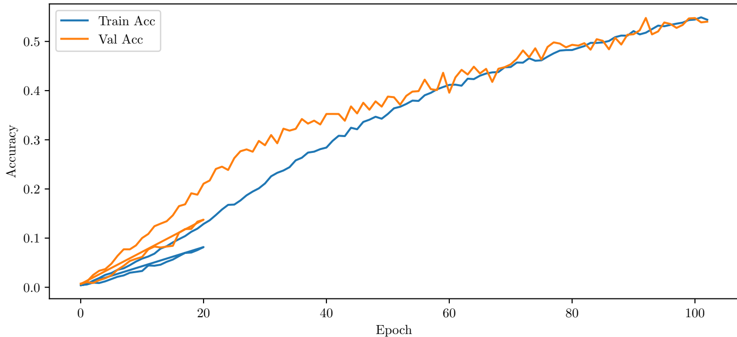
GSL Transformer — Accuracy — d_{\text{model}} = 128 — No augmentation
