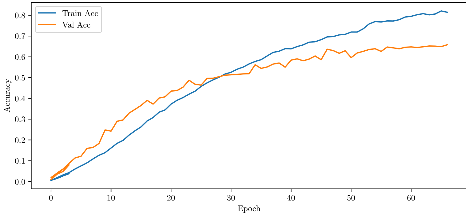
GSL Transformer — Accuracy — d_{\text{model}} = 256 — Augmentation
