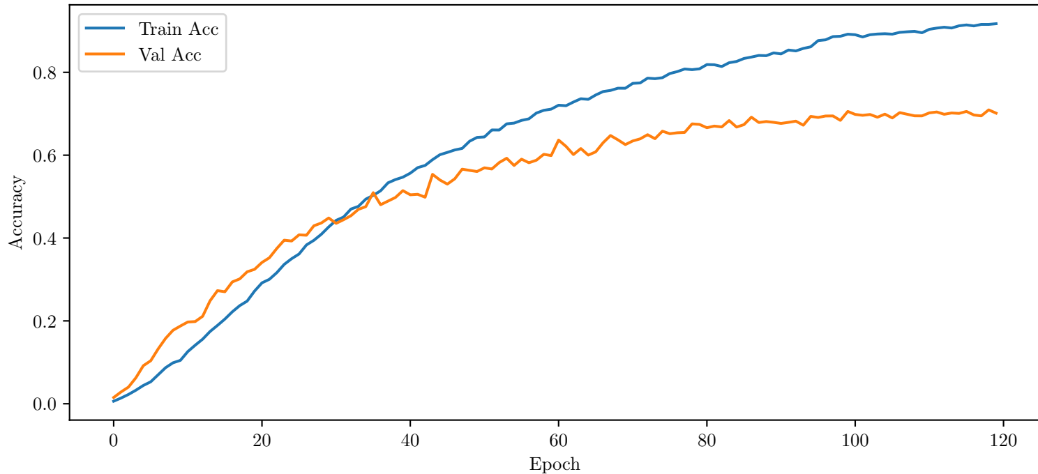
GSL Transformer — Accuracy — d_{\text{model}} = 256 — batch = 256 - ls = 0.1
