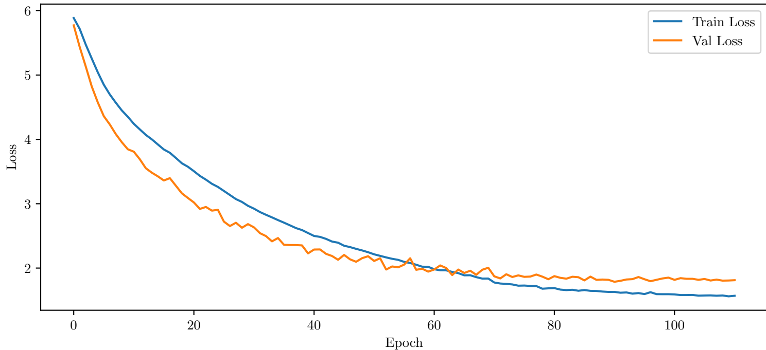
GSL Transformer — Loss - rd_{model} = 128 - Augmentation
