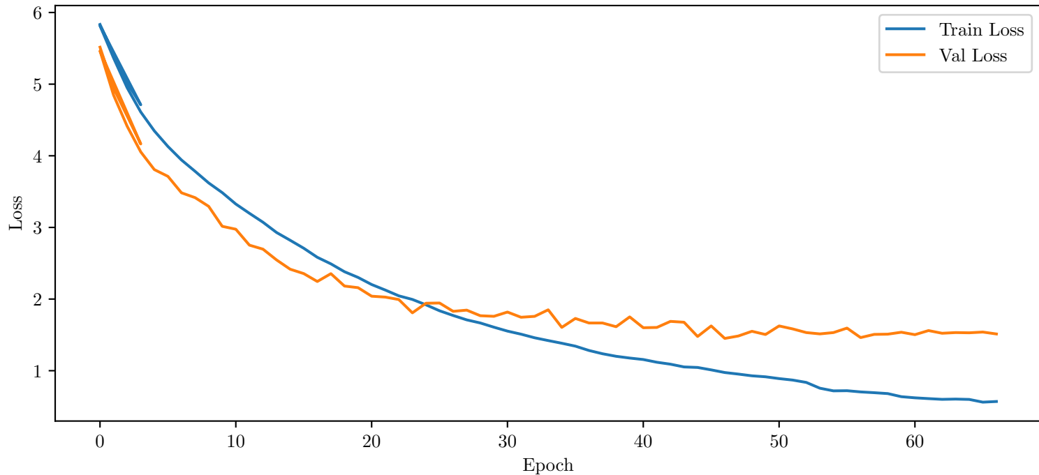
GSL Transformer — Loss - rd_{mmodel} = 256 - Augmentation
