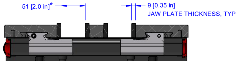
Dual Station Jaw Carriers Jaw plate stops on opposing jaw plate, typical both sides
