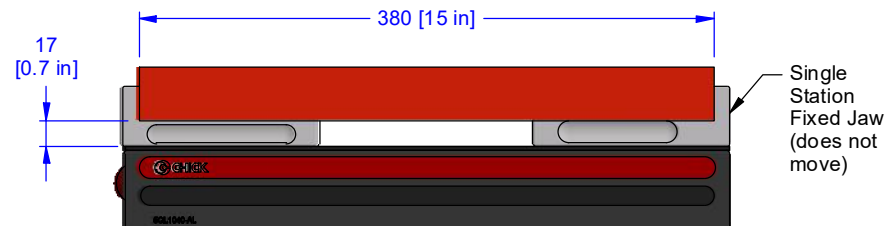
Maximum Capacity (Standard or Extended Travel Coverplate)
