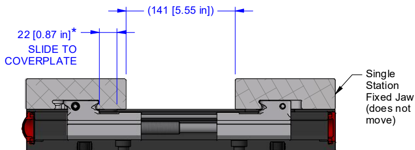
Standard Coverplate Slide stops at coverplate
