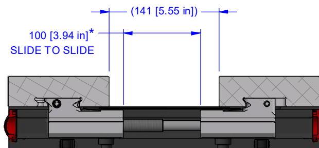
Extended Travel Coverplate Slide stops at opposing slide
