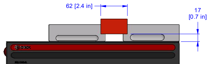
Minimum Capacity (Extended Travel Coverplate)
