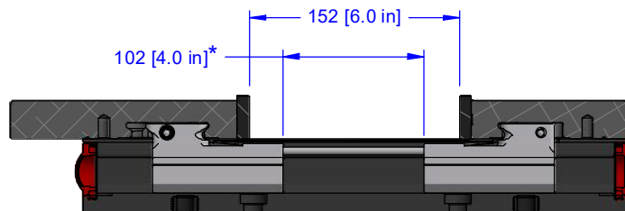
Single Station (Short Movable) Jaw Carriers Slide stops on opposing slide; Jaw plates do not close on one another
