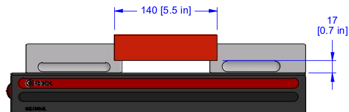
Minimum Capacity (Standard Coverplate)
