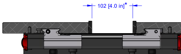
Single Station (Long Movable) Jaw Carriers Jaw plate stops on opposing jaw plate
