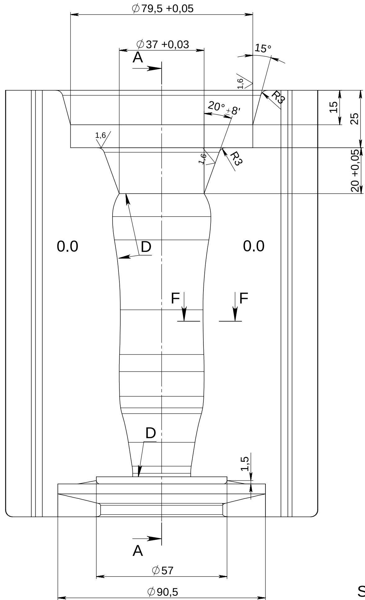
DETAIL A (FEMAIL HALF)
