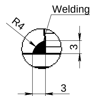
DETAIL VIEW H SCALE 2 : 1
