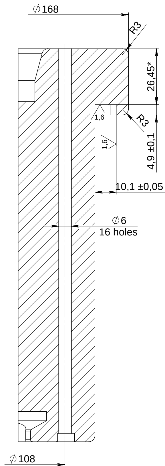
SECTION E-E
