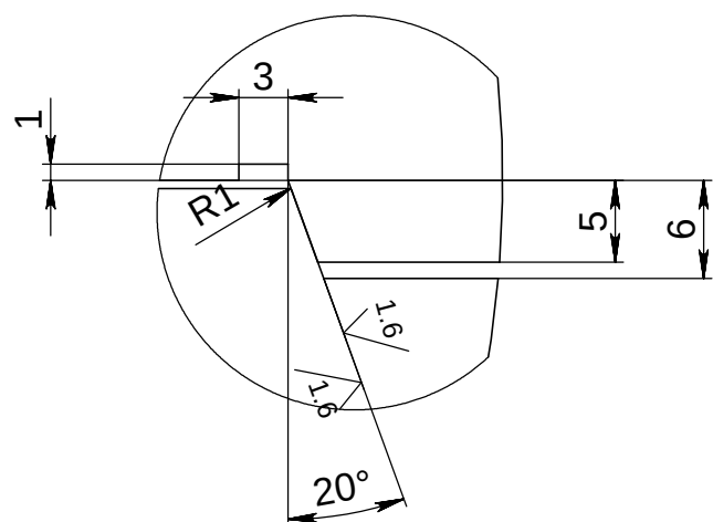
DETAIL VIEW B SCALE 2 : 1
