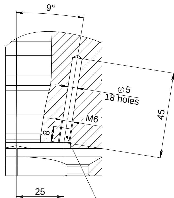
SECTION G-G
