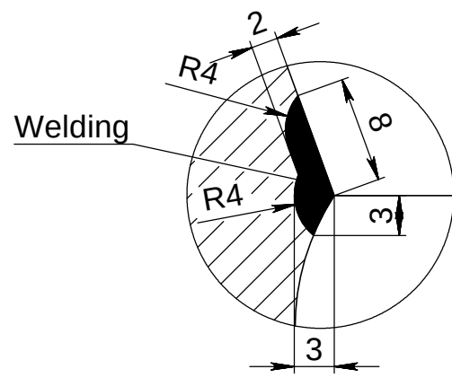
DETAIL VIEW I SCALE 2 : 1
