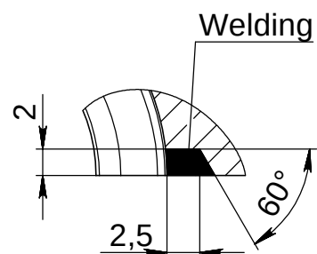
SECTION F-F SCALE 2 : 1
