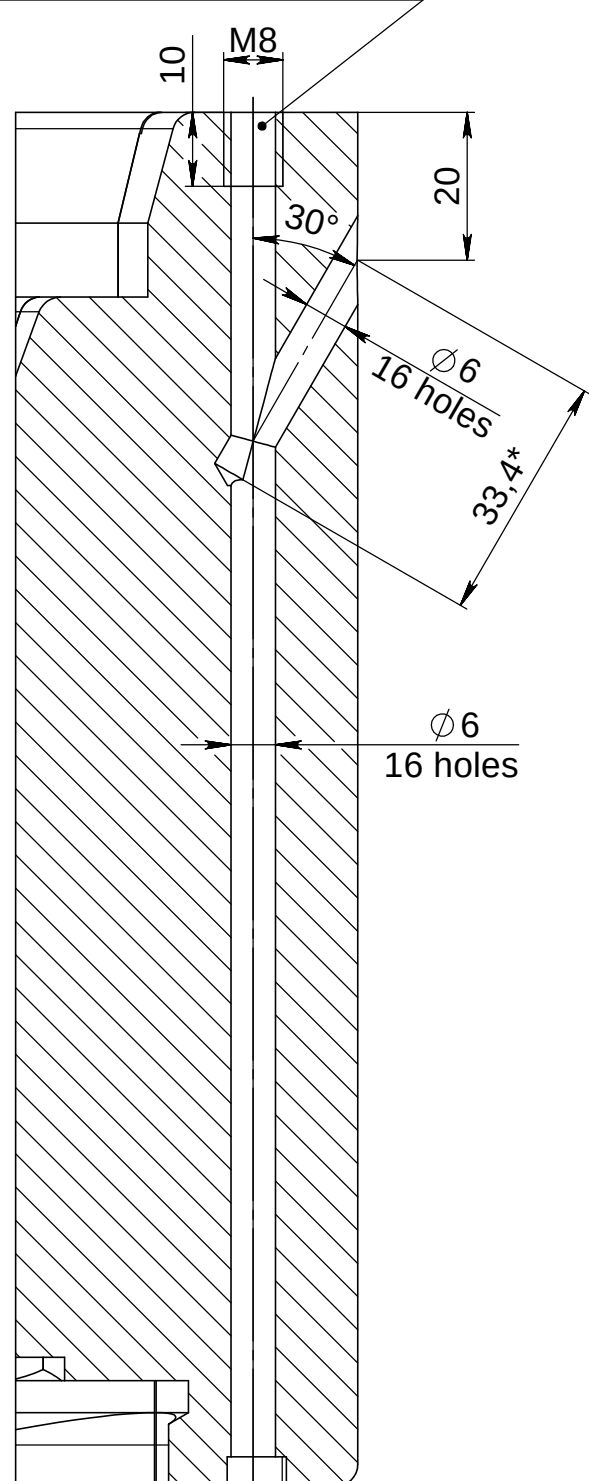
SECTION C-C
