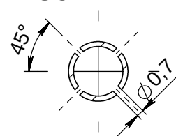
SECTION F-F SCALE 2 : 1
