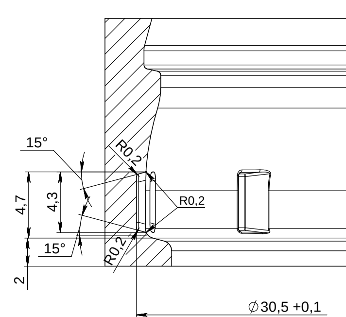
DETAIL VIEW D SCALE 8 : 1
