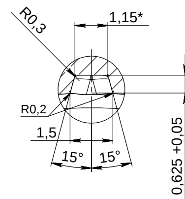
DETAIL VIEW C SCALE 8 : 1
