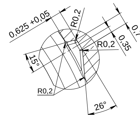
DETAIL VIEW D SCALE 8 : 1
