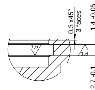
DETAIL VIEW B SCALE 2 : 1
