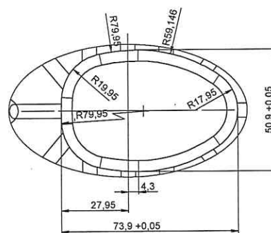
CAVITY VIEW
