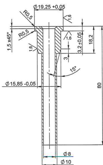
BLOWHEAD TUBE material: steel
