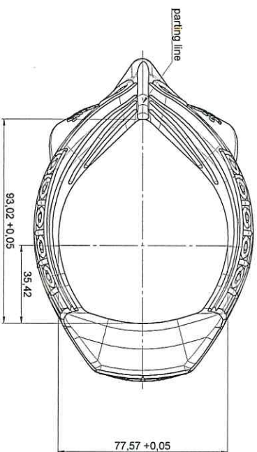
BOTTOM VIEW
