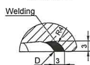
DETAIL VIEW C SCALE 2:1
