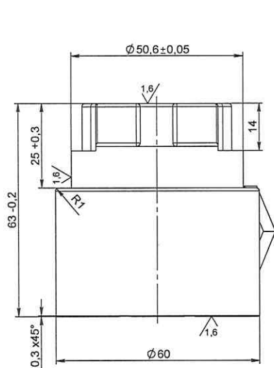
BLOWHEAD TUBE material: steel
