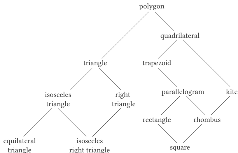
Figure 2.26: Relations among types of geometric figures.
