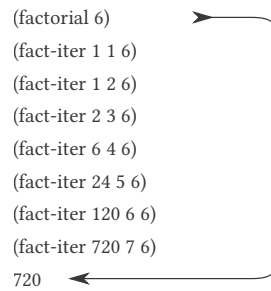
Figure 1.4: A linear iterative process for computing 6!.
