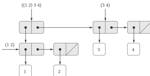
Figure 2.5: Structure formed by (cons (list 1 2) (list 3 4)) .
