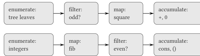
Figure 2.7: The signal-flow plans for the procedures sum-odd-squares (top) and even-fibs (bottom) reveal the commonality between the two programs.
