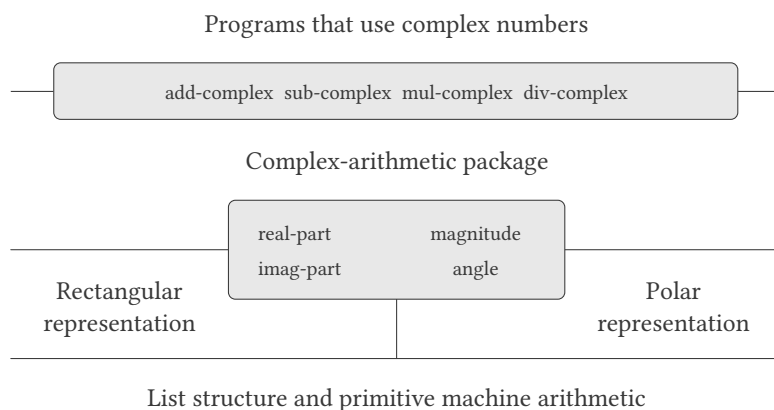
Figure 2.21: Structure of the generic complex-arithmetic system.
