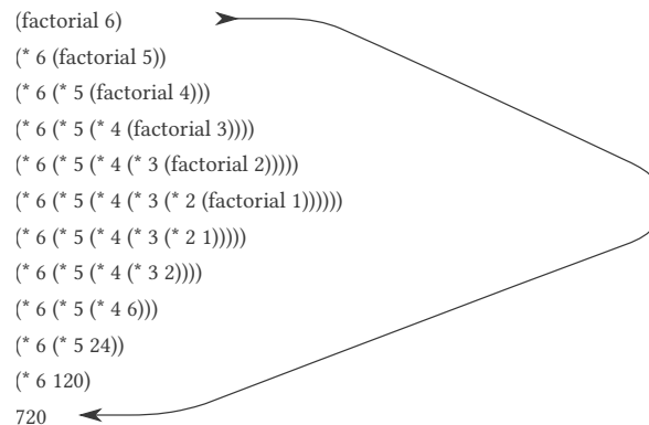
Figure 1.3: A linear recursive process for computing 6! .
