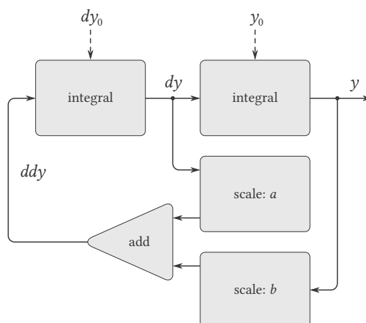
Figure 3.35: Signal-flow diagram for the solution to a second-order linear differential equation.
