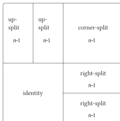
Figure 2.13: Recursive plans for right-split and corner-split.
