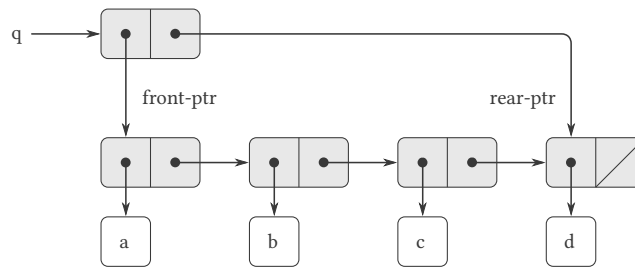
Figure 3.20: Result of using (insert-queue! q 'd) on the queue of Figure 3.19.
