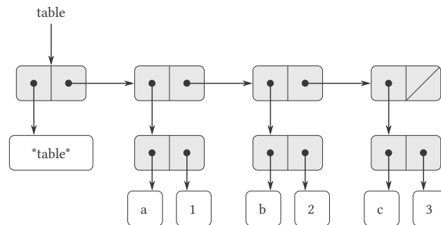
Figure 3.22: A table represented as a headed list.
