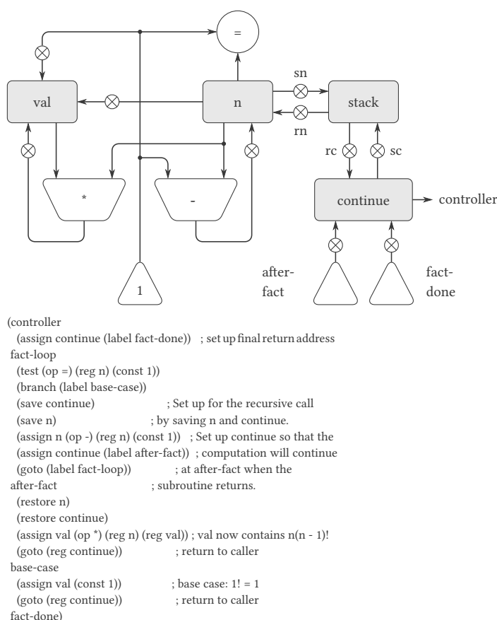
Figure 5.11: A recursive factorial machine.
