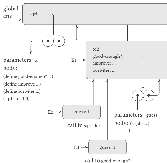
Figure 3.11: Sqrt procedure with internal definitions.
