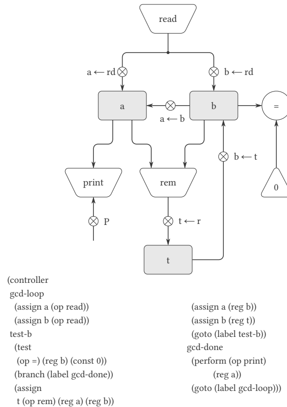
Figure 5.4: A GCD machine that reads inputs and prints results.
