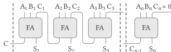
Figure 3.27: A ripple-carry adder for n -bit numbers.
