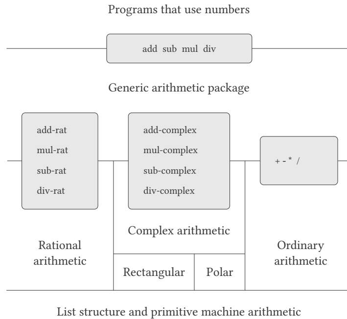
Figure 2.23: Generic arithmetic system.
