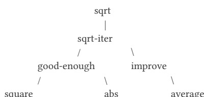
Figure 1.2: Procedural decomposition of the sqrt program.
