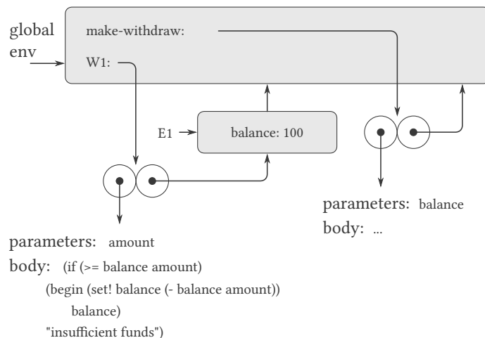
Figure 3.7: Result of evaluating (define W1 (make-withdraw 100)) .
