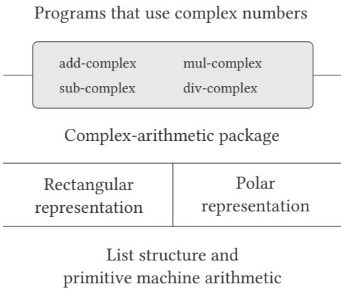
Figure 2.19: Data-abstraction barriers in the complex-number system.
