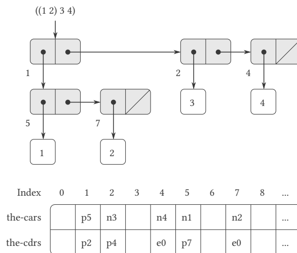
Figure 5.14: Box-and-pointer and memory-vector representations of the list ((1 2) 3 4) .
