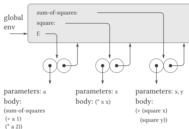
Figure 3.4: Procedure objects in the global frame.
