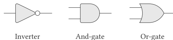
Figure 3.24: Primitive functions in the digital logic simulator.
