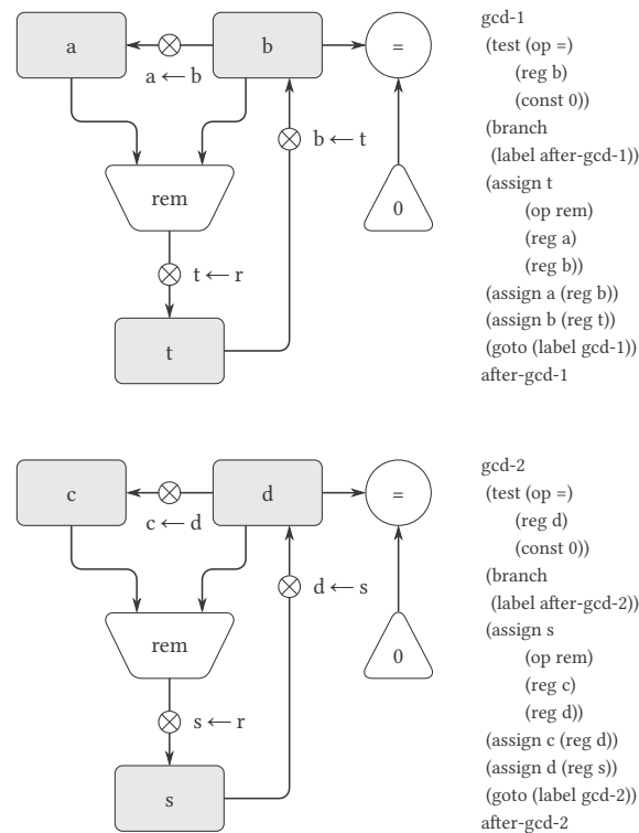
Figure 5.7: Portions of the data paths and controller sequence for a machine with two GCD computations.
