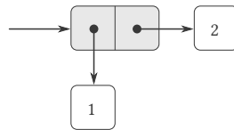
Figure 2.2: Box-and-pointer representation of (cons 1 2) .
