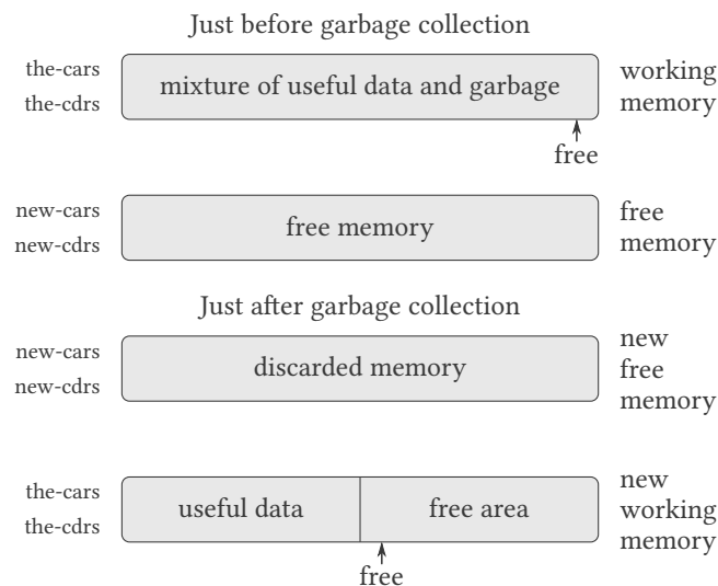
Figure 5.15: Reconfiguration of memory by the garbage-collection process.
