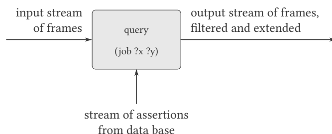
Figure 4.4: A query processes a stream of frames.
