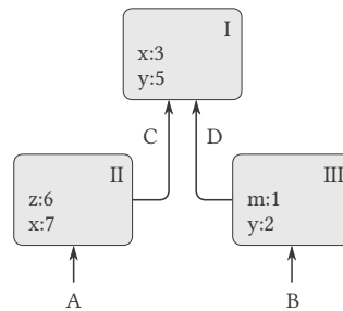
Figure 3.1: A simple environment structure.
