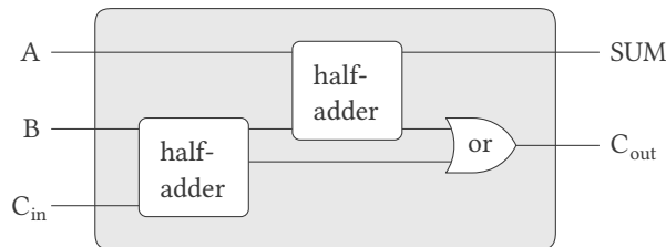
Figure 3.26: A full-adder circuit.
