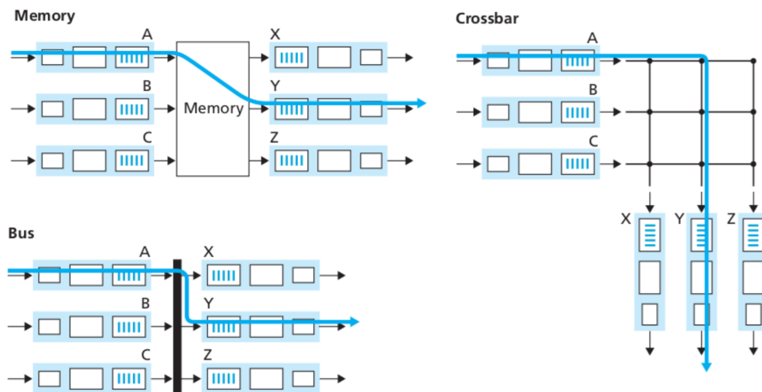
Figure 3.3. The three types of switching fabric.
