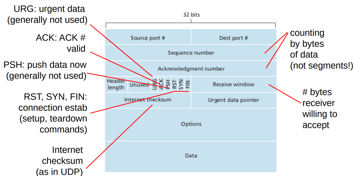
The structure of a TCP segment.
