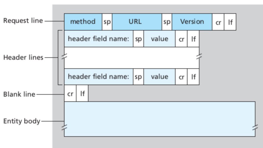
General format of a HTTP request message.
