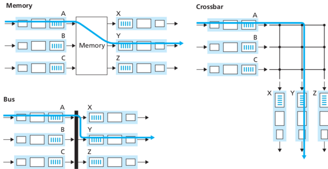
Figure 3.2. The three types of switching fabric.
