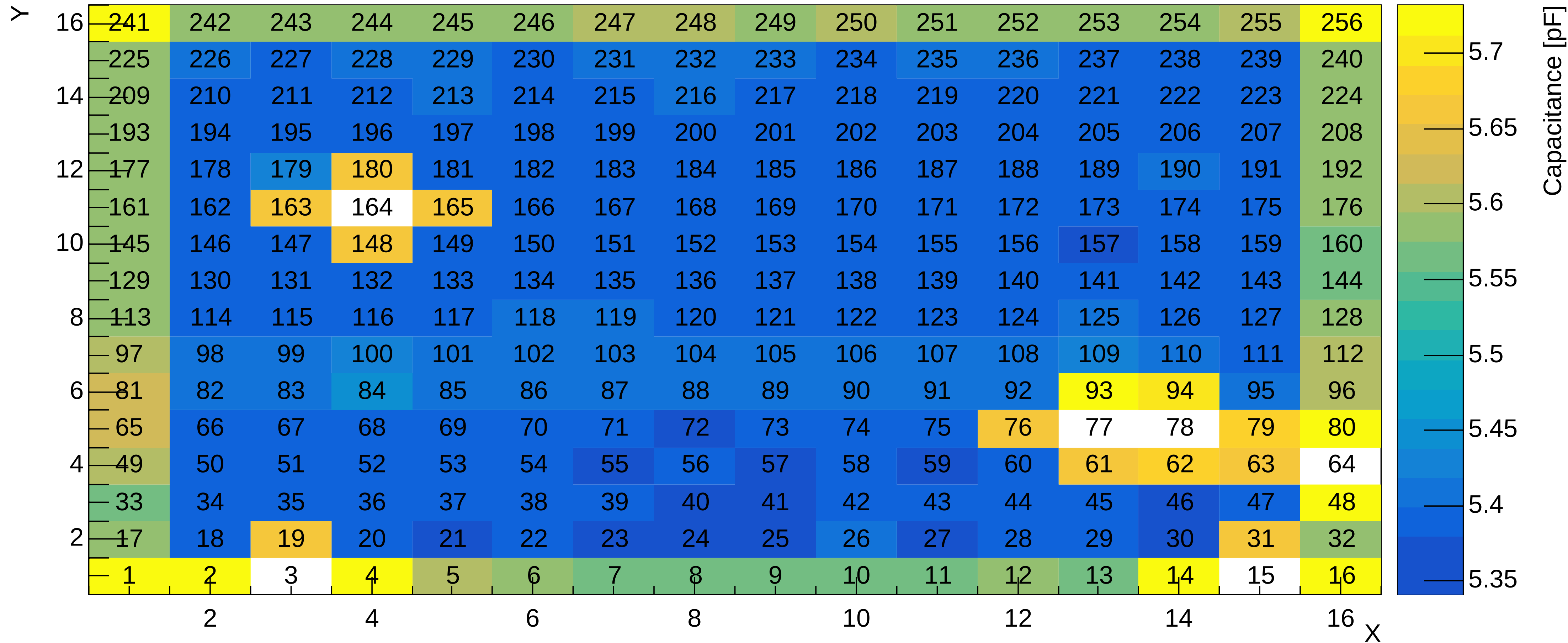
Full depletion capacitance for sensor 16
