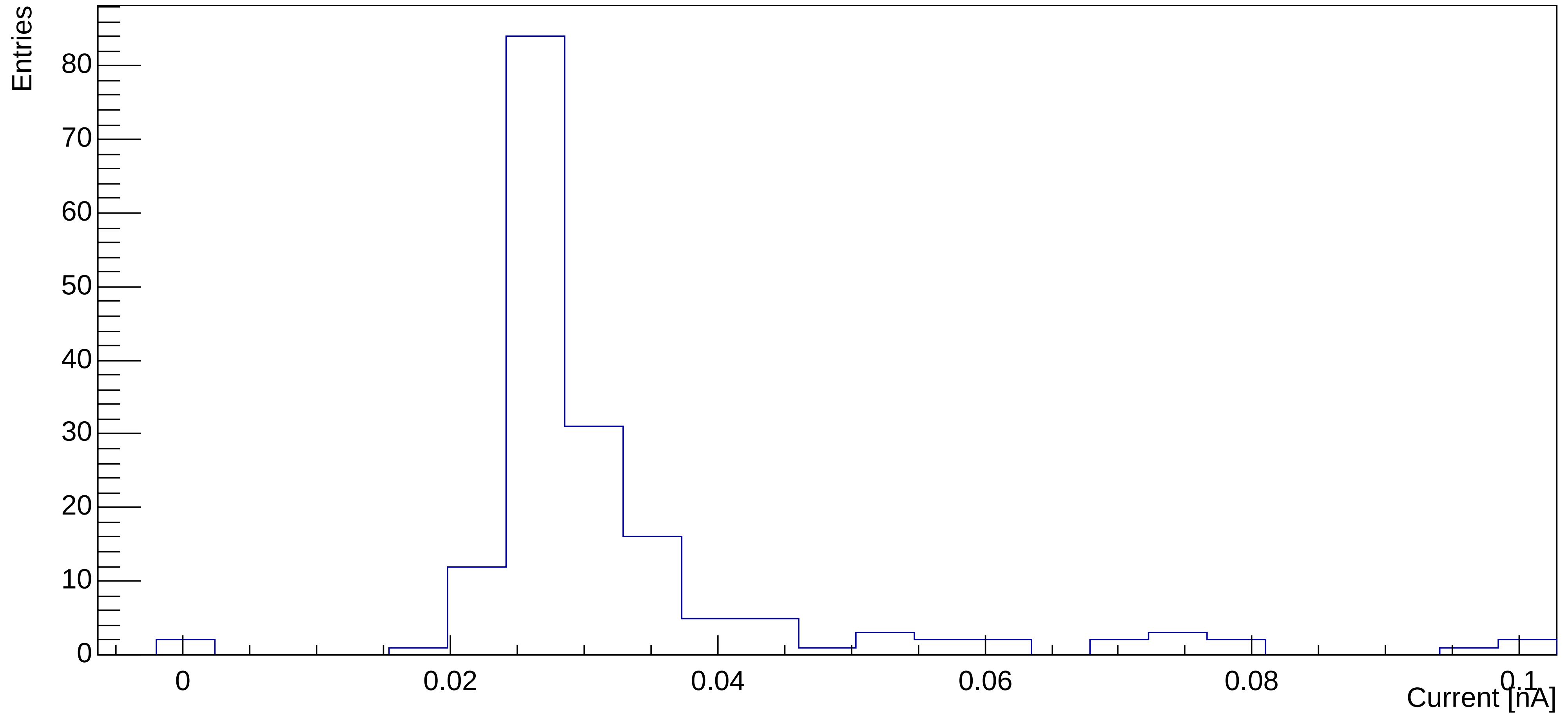
Current distribution in inner channels zoomed
